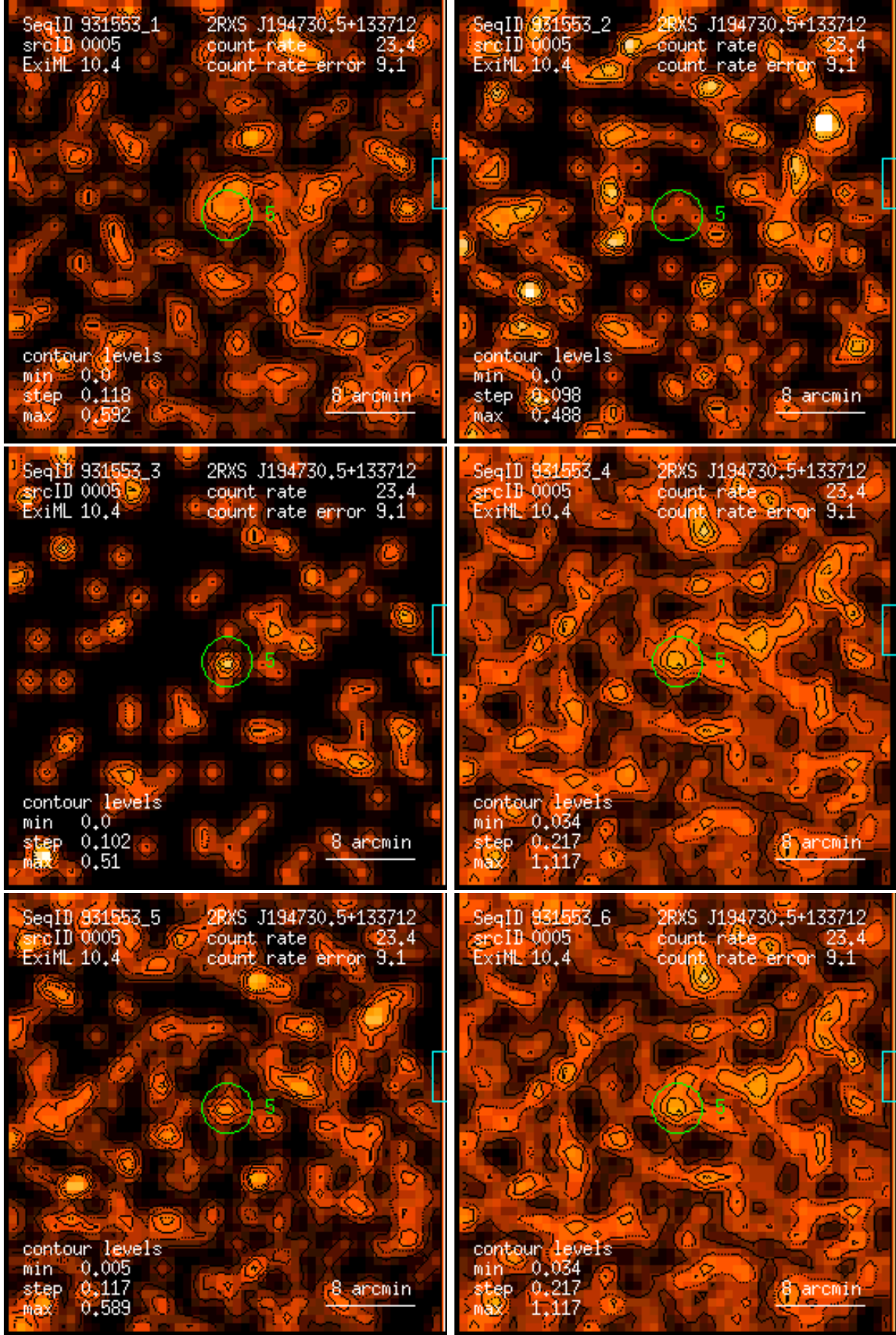
Figure 5: RASS 931553: detection 0005: band rate images, Gaussian filter: (1) PSPC channels 11 – 41, (2) 52 – 90, (3) 91 – 201, (4) 11 – 235, (5) 52 – 201, (6) 11 – 201. Broad band rates in counts/ks. Band rate contour levels in counts/ks/arcmin 2 .
