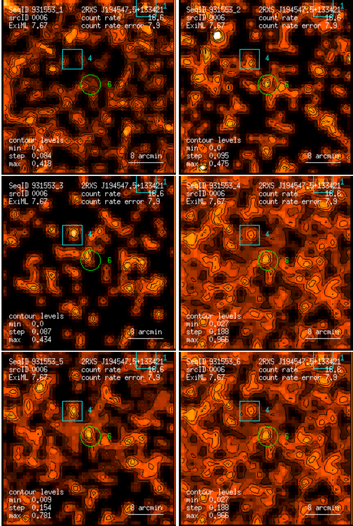
Figure 6: RASS 931553: detection 0006: band rate images, Gaussian filter: (1) PSPC channels 11 – 41, (2) 52 – 90, (3) 91 – 201, (4) 11 – 235, (5) 52 – 201, (6) 11 – 201. Broad band rates in counts/ks. Band rate contour levels in counts/ks/arcmin 2 .
