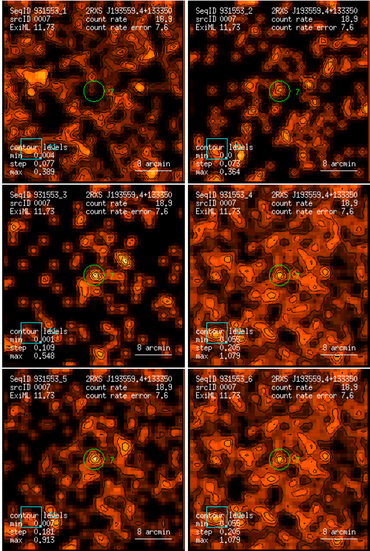
Figure 7: RASS 931553: detection 0007: band rate images, Gaussian filter: (1) PSPC channels 11 – 41, (2) 52 – 90, (3) 91 – 201, (4) 11 – 235, (5) 52 – 201, (6) 11 – 201. Broad band rates in counts/ks. Band rate contour levels in counts/ks/arcmin 2 .
