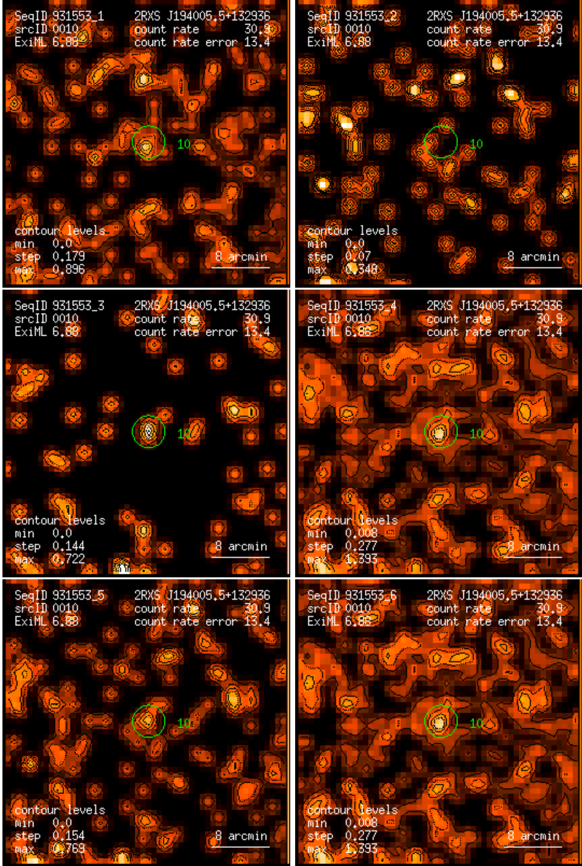
Figure 10: RASS 931553: detection 0010: band rate images, Gaussian filter: (1) PSPC channels 11 – 41, (2) 52 – 90, (3) 91 – 201, (4) 11 – 235, (5) 52 – 201, (6) 11 – 201. Broad band rates in counts/ks. Band rate contour levels in counts/ks/arcmin 2 .
