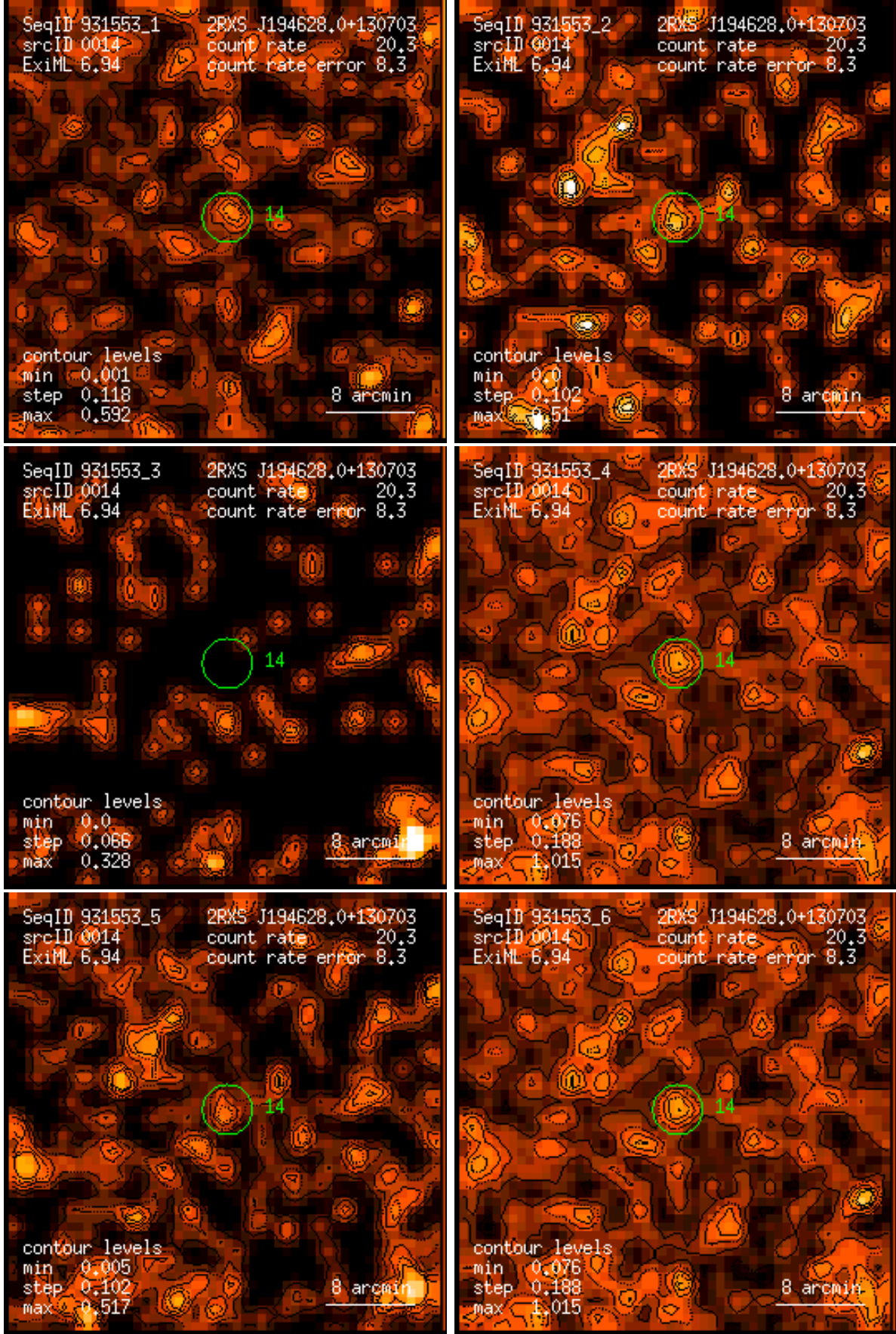
Figure 14: RASS 931553: detection 0014: band rate images, Gaussian filter: (1) PSPC channels 11 – 41, (2) 52 – 90, (3) 91 – 201, (4) 11 – 235, (5) 52 – 201, (6) 11 – 201. Broad band rates in counts/ks. Band rate contour levels in counts/ks/arcmin 2 .
