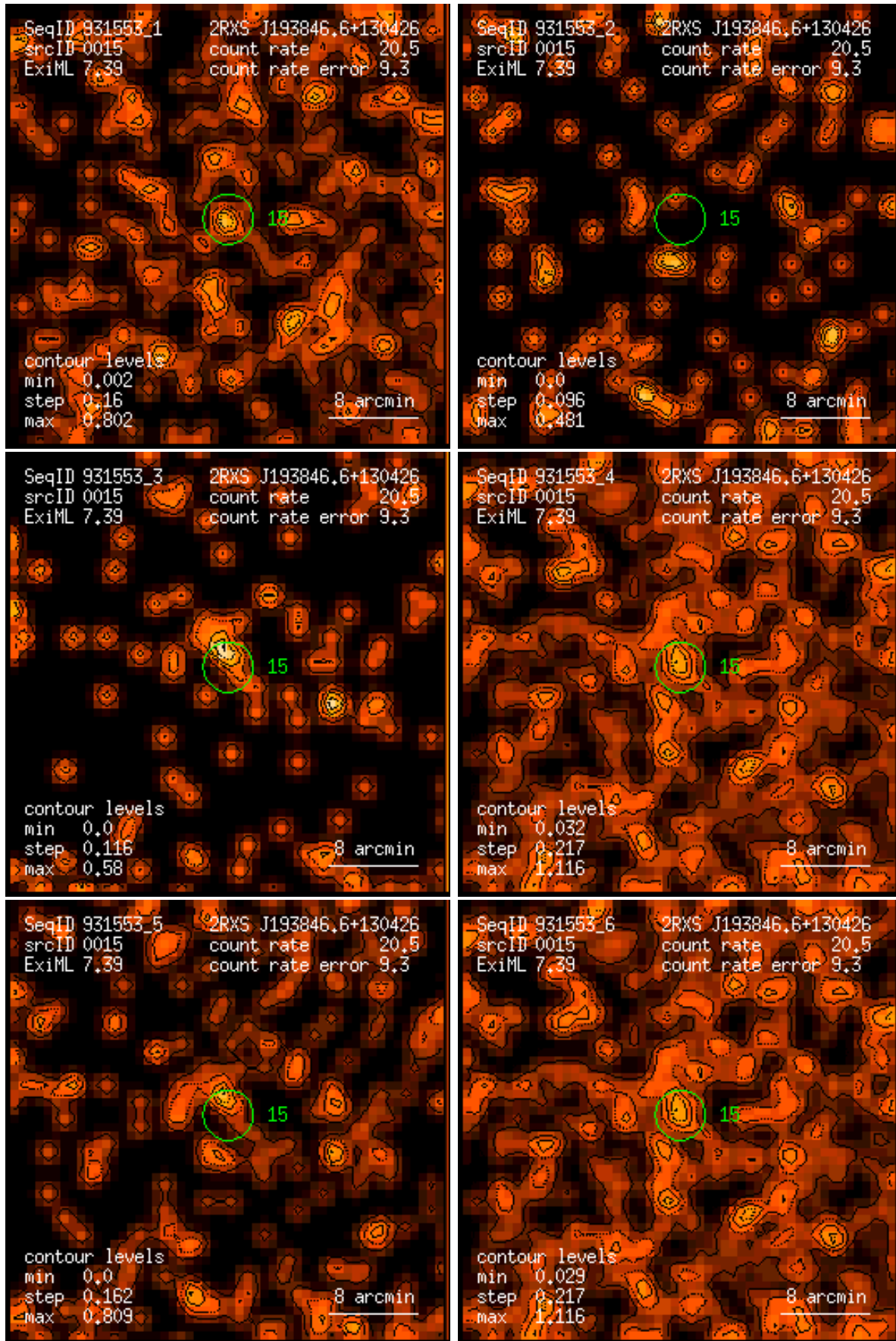
Figure 15: RASS 931553: detection 0015: band rate images, Gaussian filter: (1) PSPC channels 11 – 41, (2) 52 – 90, (3) 91 – 201, (4) 11 – 235, (5) 52 – 201, (6) 11 – 201. Broad band rates in counts/ks. Band rate contour levels in counts/ks/arcmin 2 .
