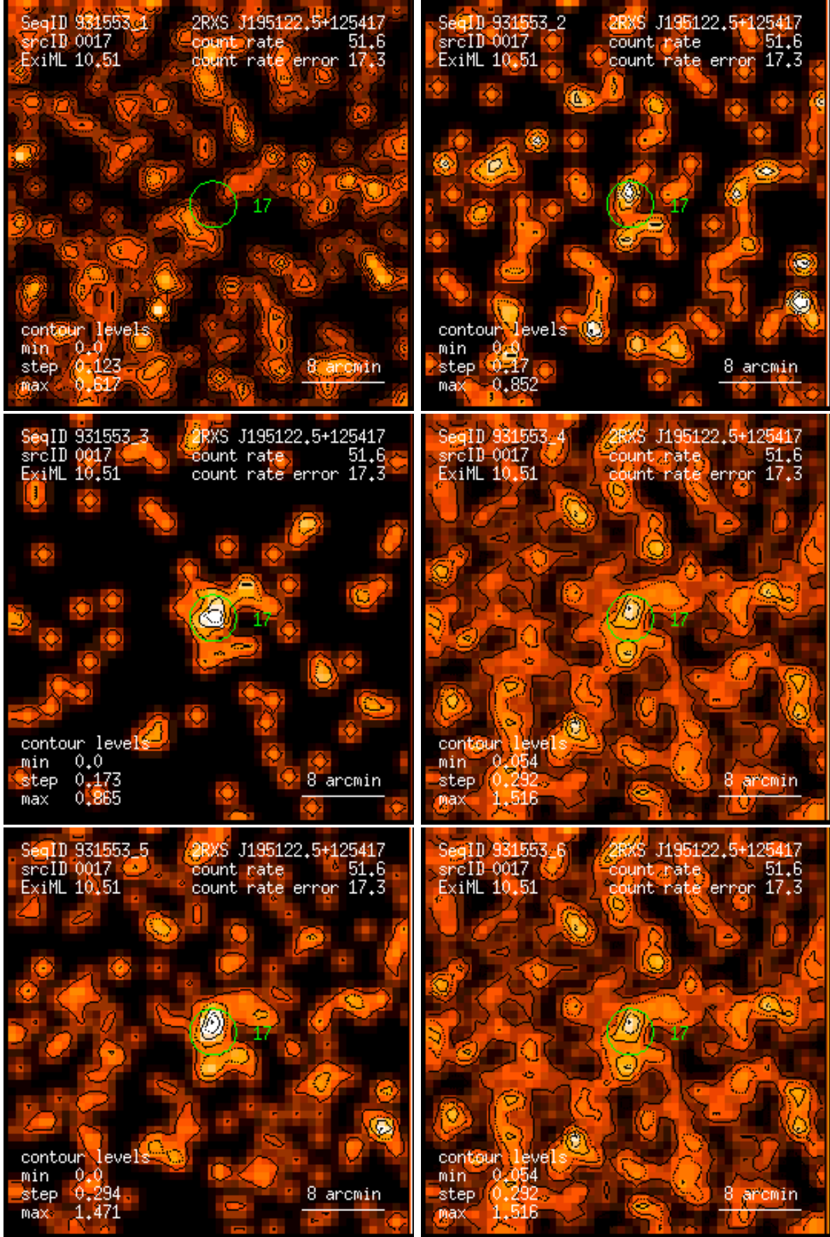
Figure 17: RASS 931553: detection 0017: band rate images, Gaussian filter: (1) PSPC channels 11 – 41, (2) 52 – 90, (3) 91 – 201, (4) 11 – 235, (5) 52 – 201, (6) 11 – 201. Broad band rates in counts/ks. Band rate contour levels in counts/ks/arcmin 2 .
