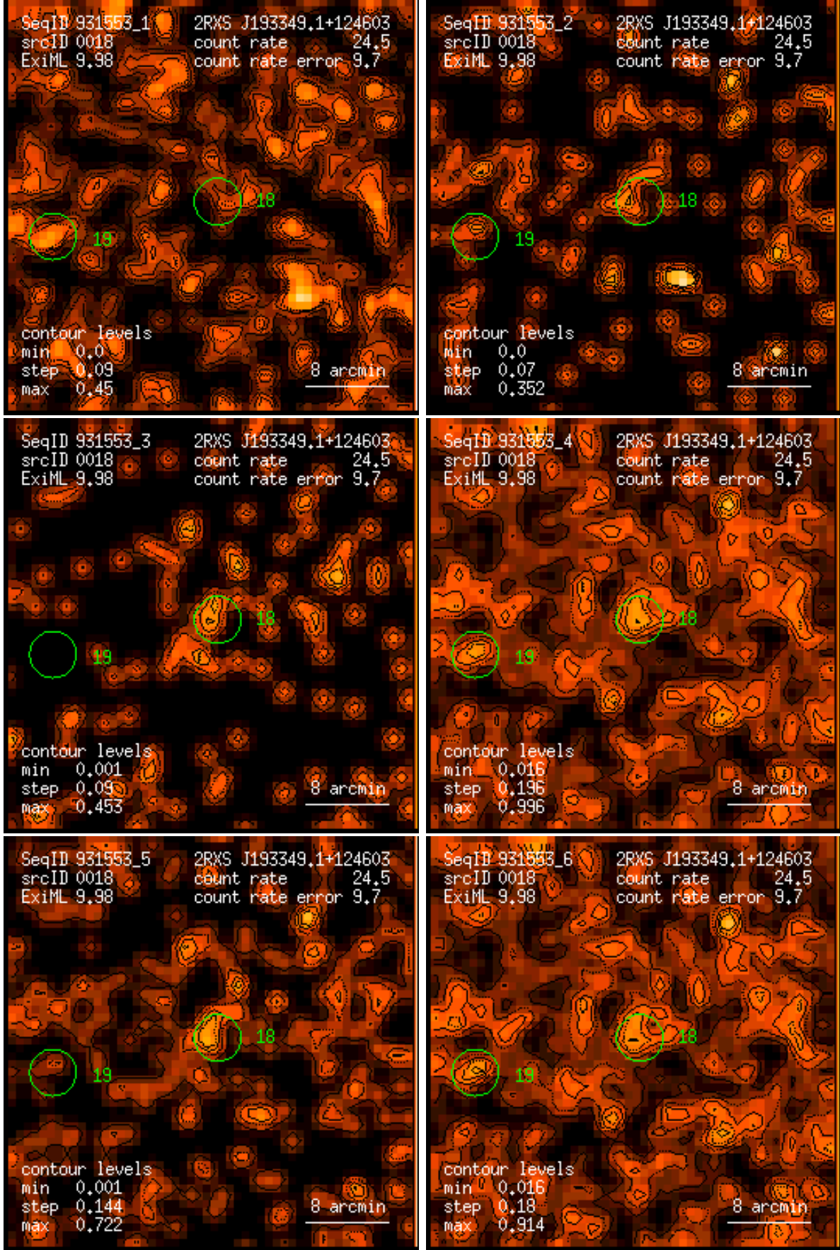
Figure 18: RASS 931553: detection 0018: band rate images, Gaussian filter: (1) PSPC channels 11 – 41, (2) 52 – 90, (3) 91 – 201, (4) 11 – 235, (5) 52 – 201, (6) 11 – 201. Broad band rates in counts/ks. Band rate contour levels in counts/ks/arcmin 2 .
