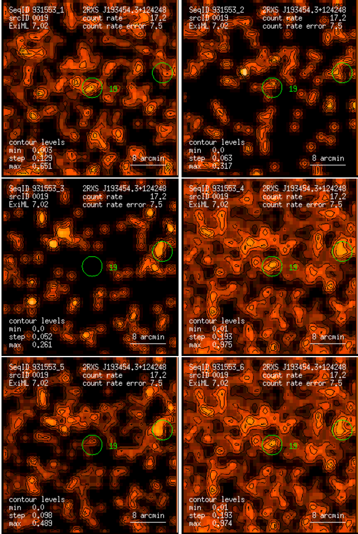
Figure 19: RASS 931553: detection 0019: band rate images, Gaussian filter: (1) PSPC channels 11 – 41, (2) 52 – 90, (3) 91 – 201, (4) 11 – 235, (5) 52 – 201, (6) 11 – 201. Broad band rates in counts/ks. Band rate contour levels in counts/ks/arcmin 2 .
