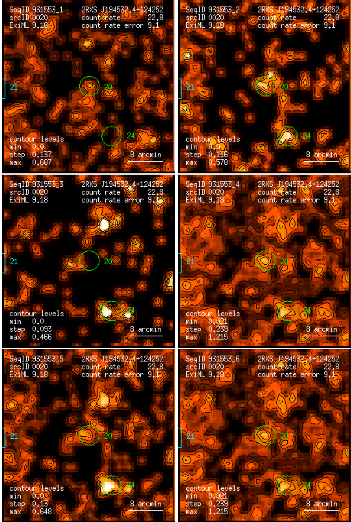
Figure 20: RASS 931553: detection 0020: band rate images, Gaussian filter: (1) PSPC channels 11 – 41, (2) 52 – 90, (3) 91 – 201, (4) 11 – 235, (5) 52 – 201, (6) 11 – 201. Broad band rates in counts/ks. Band rate contour levels in counts/ks/arcmin 2 .
