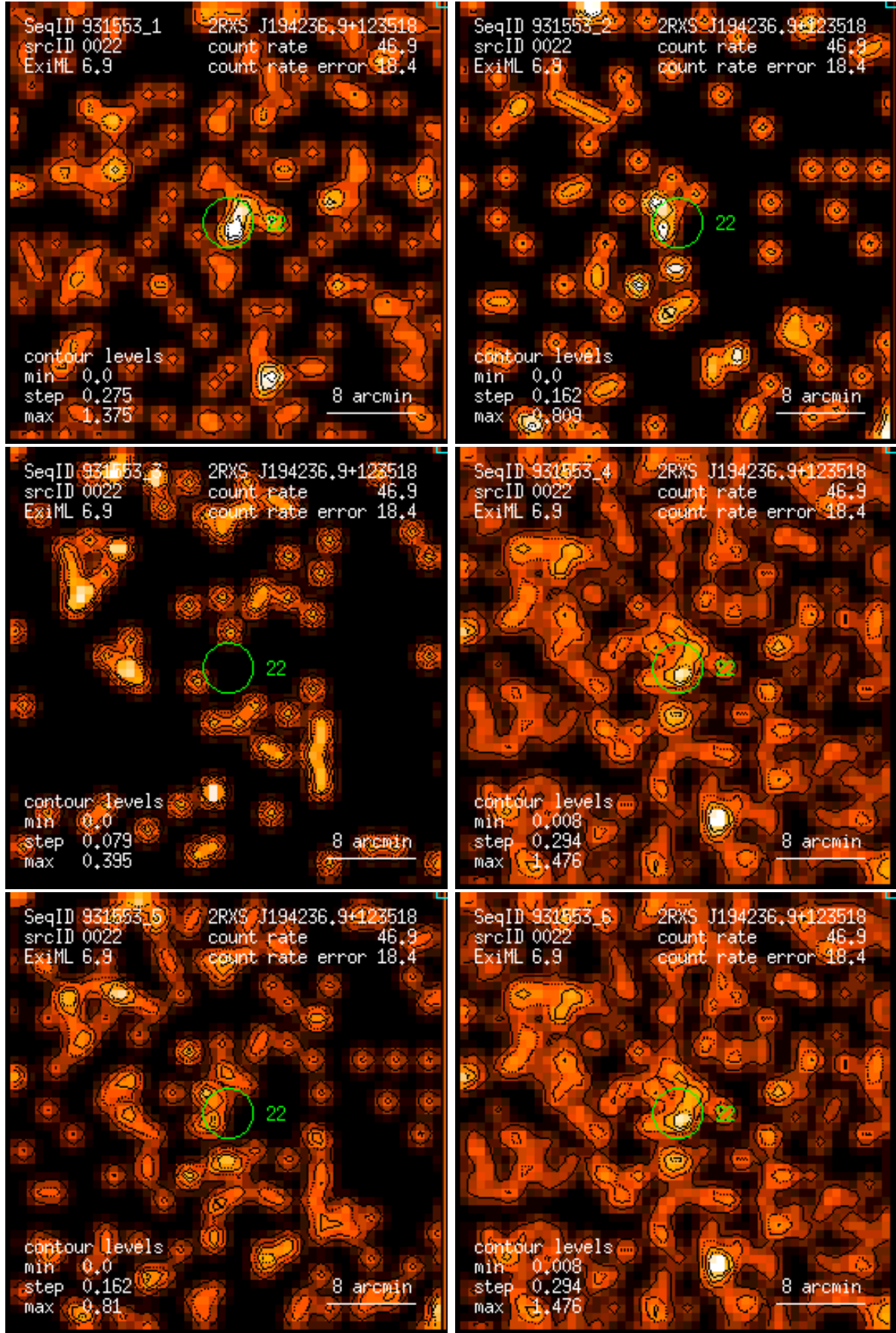
Figure 22: RASS 931553: detection 0022: band rate images, Gaussian filter: (1) PSPC channels 11 – 41, (2) 52 – 90, (3) 91 – 201, (4) 11 – 235, (5) 52 – 201, (6) 11 – 201. Broad band rates in counts/ks. Band rate contour levels in counts/ks/arcmin 2 .
