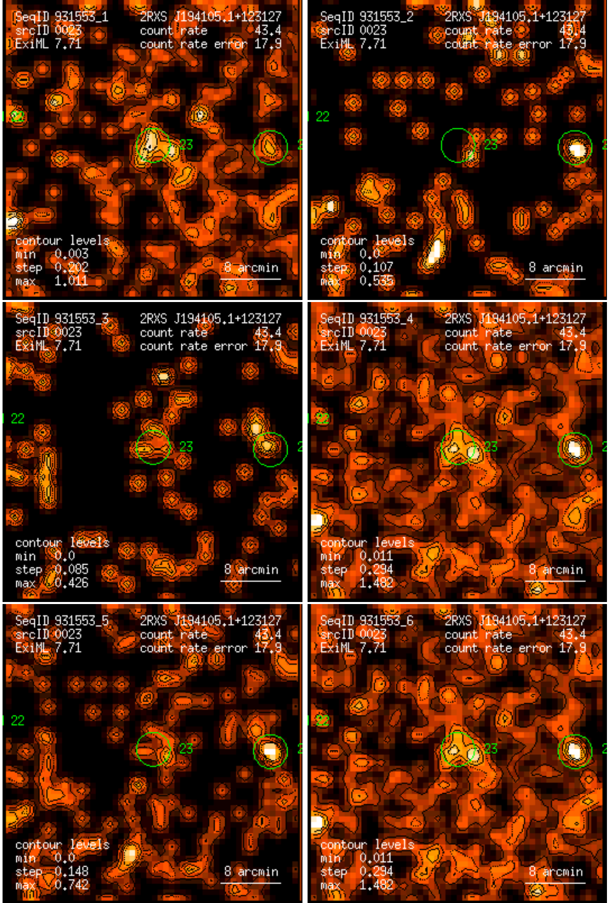
Figure 23: RASS 931553: detection 0023: band rate images, Gaussian filter: (1) PSPC channels 11 – 41, (2) 52 – 90, (3) 91 – 201, (4) 11 – 235, (5) 52 – 201, (6) 11 – 201. Broad band rates in counts/ks. Band rate contour levels in counts/ks/arcmin 2 .
