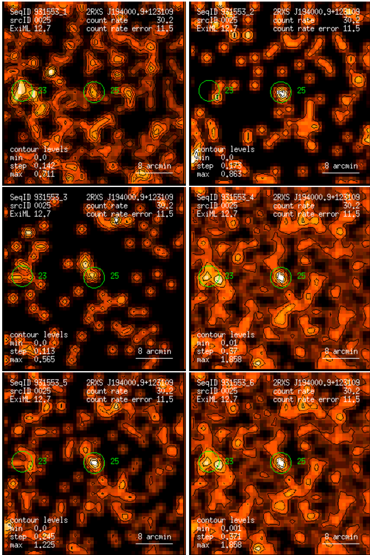
Figure 25: RASS 931553: detection 0025: band rate images, Gaussian filter: (1) PSPC channels 11 – 41, (2) 52 – 90, (3) 91 – 201, (4) 11 – 235, (5) 52 – 201, (6) 11 – 201. Broad band rates in counts/ks. Band rate contour levels in counts/ks/arcmin 2 .
