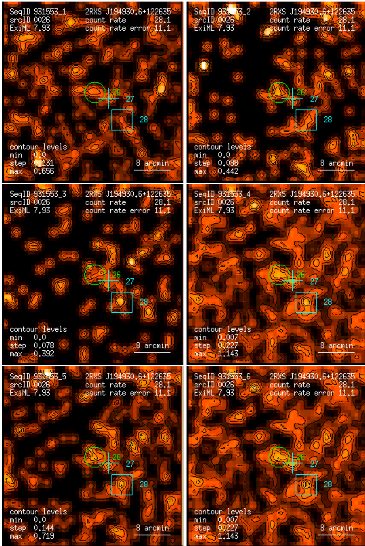
Figure 26: RASS 931553: detection 0026: band rate images, Gaussian filter: (1) PSPC channels 11 – 41, (2) 52 – 90, (3) 91 – 201, (4) 11 – 235, (5) 52 – 201, (6) 11 – 201. Broad band rates in counts/ks. Band rate contour levels in counts/ks/arcmin 2 .
