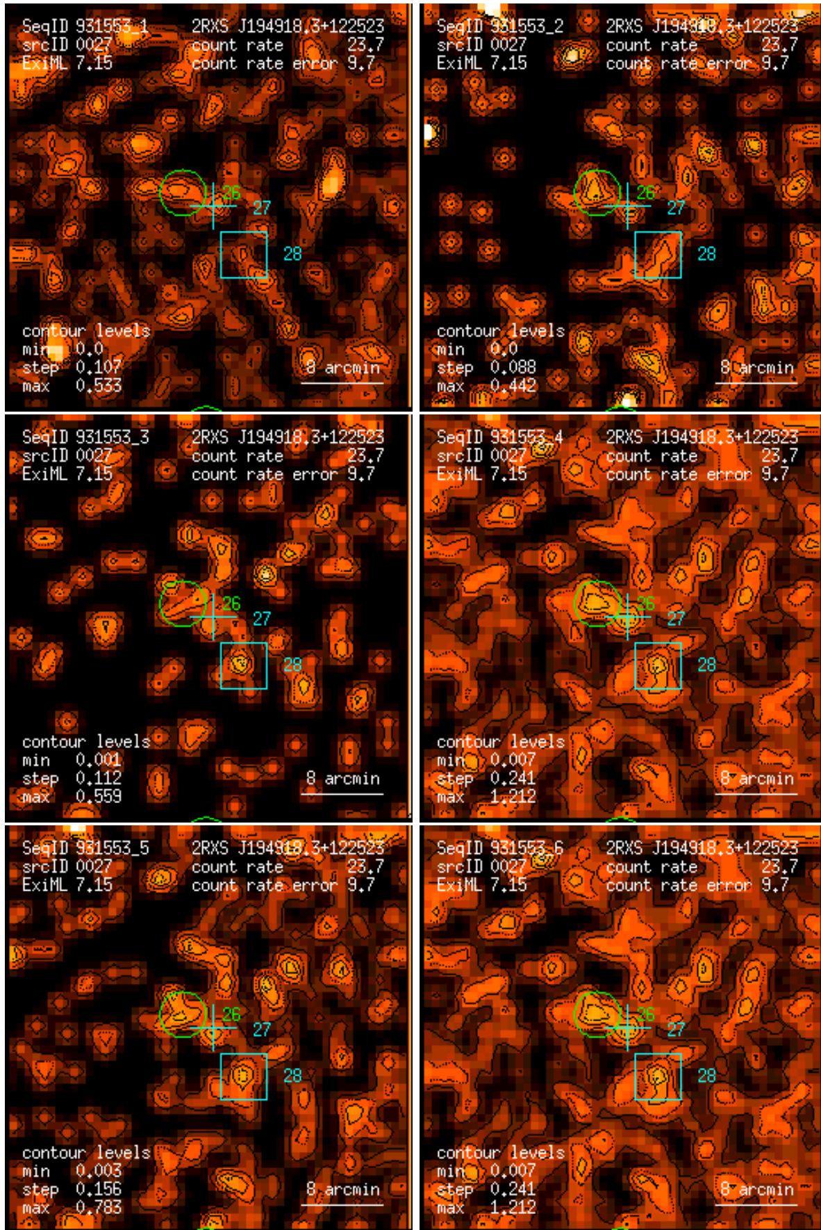
Figure 27: RASS 931553: detection 0027: band rate images, Gaussian filter: (1) PSPC channels 11 – 41, (2) 52 – 90, (3) 91 – 201, (4) 11 – 235, (5) 52 – 201, (6) 11 – 201. Broad band rates in counts/ks. Band rate contour levels in counts/ks/arcmin 2 .
