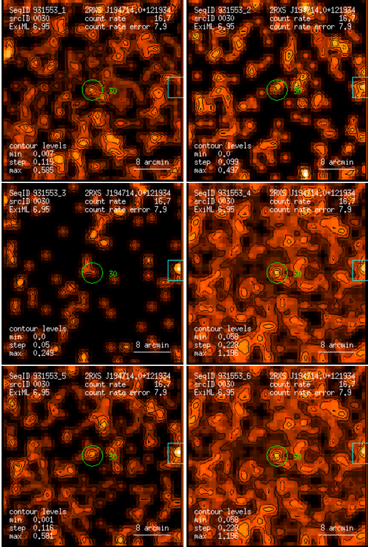
Figure 30: RASS 931553: detection 0030: band rate images, Gaussian filter: (1) PSPC channels 11 – 41, (2) 52 – 90, (3) 91 – 201, (4) 11 – 235, (5) 52 – 201, (6) 11 – 201. Broad band rates in counts/ks. Band rate contour levels in counts/ks/arcmin 2 .
