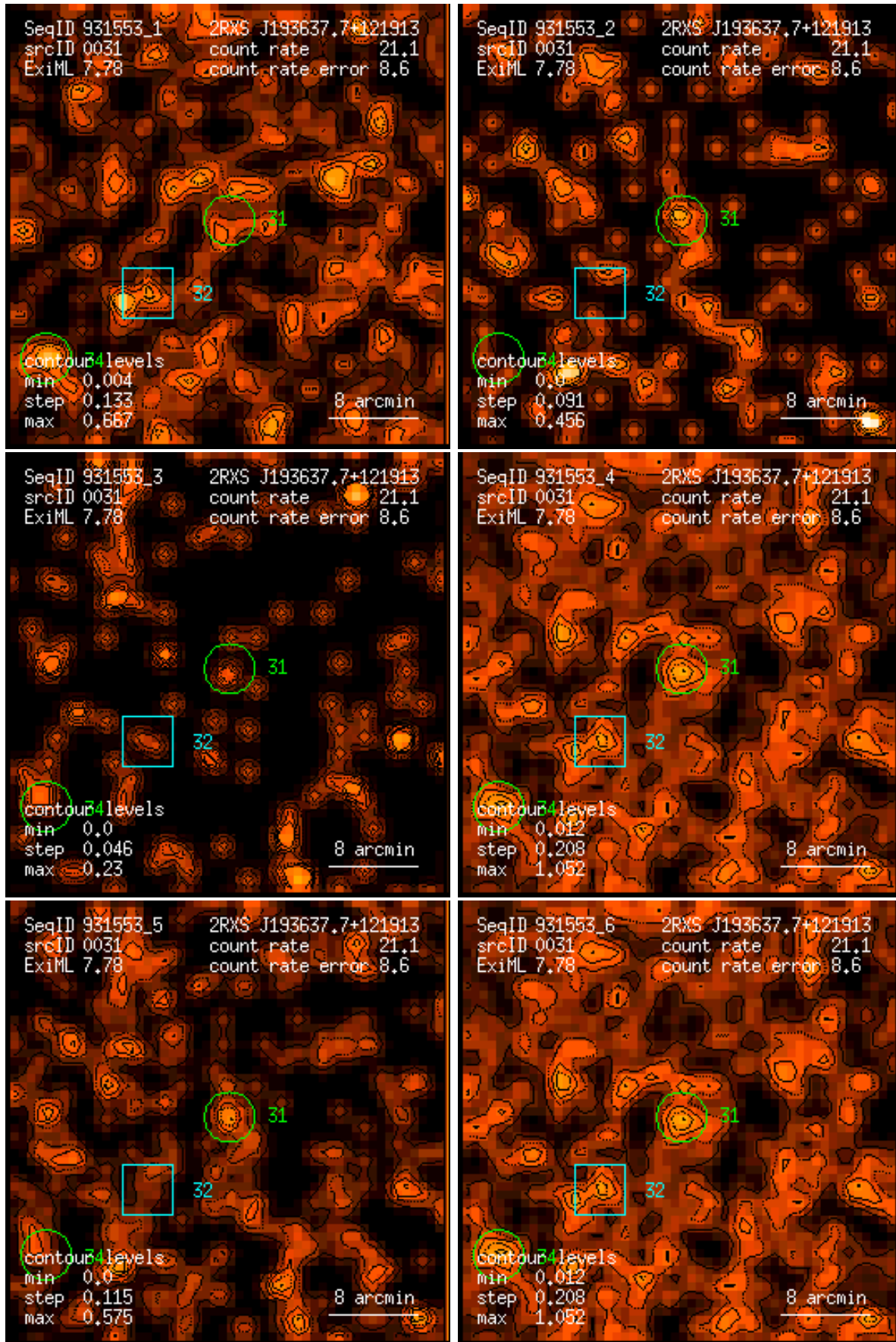
Figure 31: RASS 931553: detection 0031: band rate images, Gaussian filter: (1) PSPC channels 11 – 41, (2) 52 – 90, (3) 91 – 201, (4) 11 – 235, (5) 52 – 201, (6) 11 – 201. Broad band rates in counts/ks. Band rate contour levels in counts/ks/arcmin 2 .
