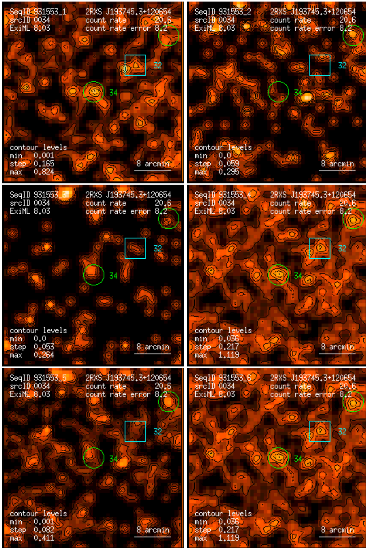
Figure 34: RASS 931553: detection 0034: band rate images, Gaussian filter: (1) PSPC channels 11 – 41, (2) 52 – 90, (3) 91 – 201, (4) 11 – 235, (5) 52 – 201, (6) 11 – 201. Broad band rates in counts/ks. Band rate contour levels in counts/ks/arcmin 2 .
