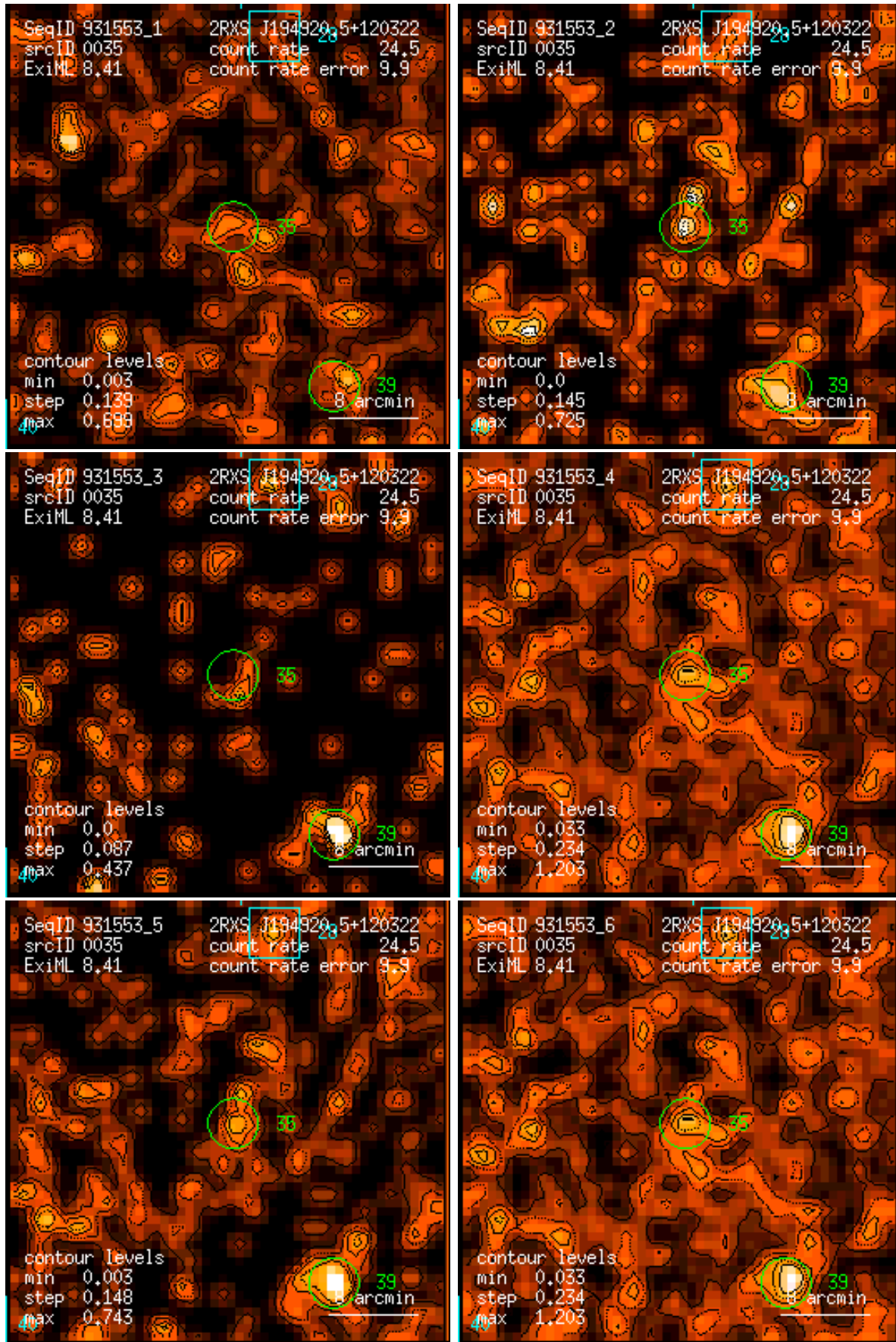
Figure 35: RASS 931553: detection 0035: band rate images, Gaussian filter: (1) PSPC channels 11 – 41, (2) 52 – 90, (3) 91 – 201, (4) 11 – 235, (5) 52 – 201, (6) 11 – 201. Broad band rates in counts/ks. Band rate contour levels in counts/ks/arcmin 2 .
