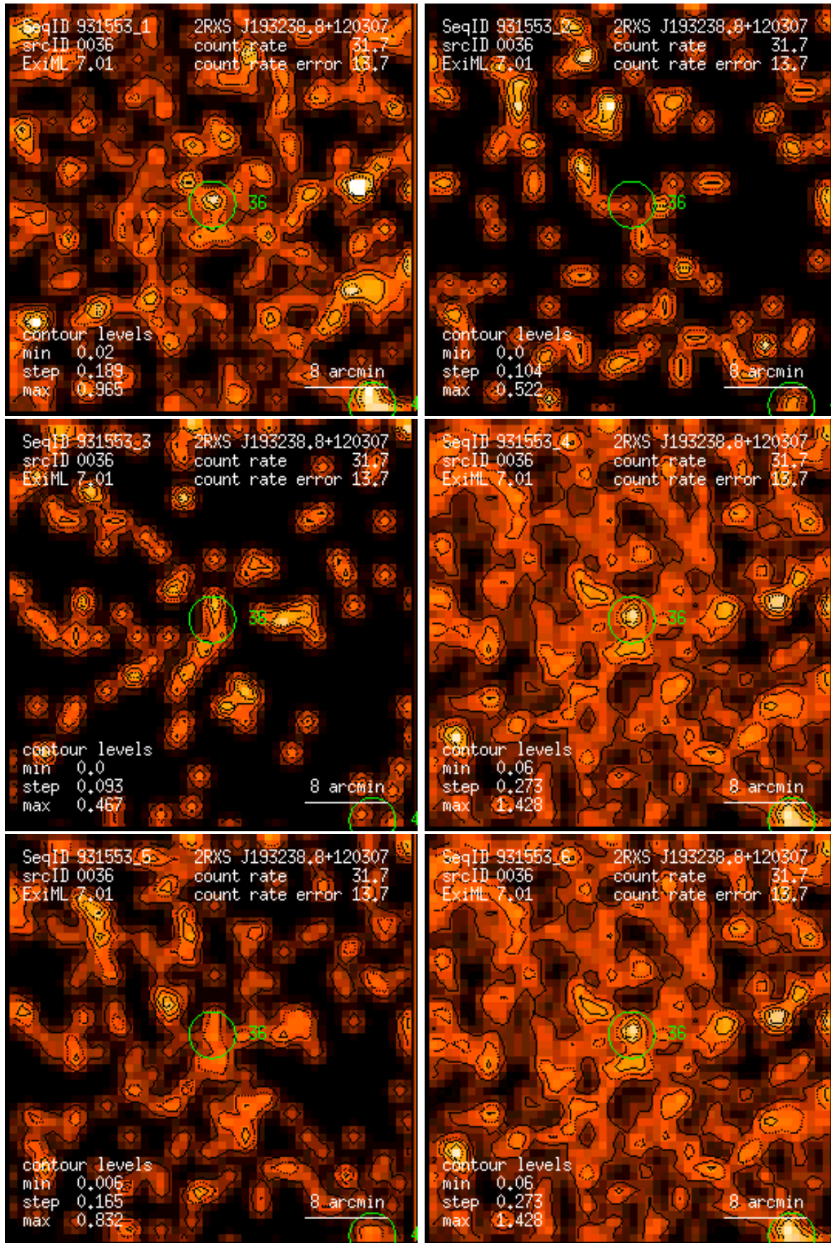
Figure 36: RASS 931553: detection 0036: band rate images, Gaussian filter: (1) PSPC channels 11 – 41, (2) 52 – 90, (3) 91 – 201, (4) 11 – 235, (5) 52 – 201, (6) 11 – 201. Broad band rates in counts/ks. Band rate contour levels in counts/ks/arcmin 2 .
