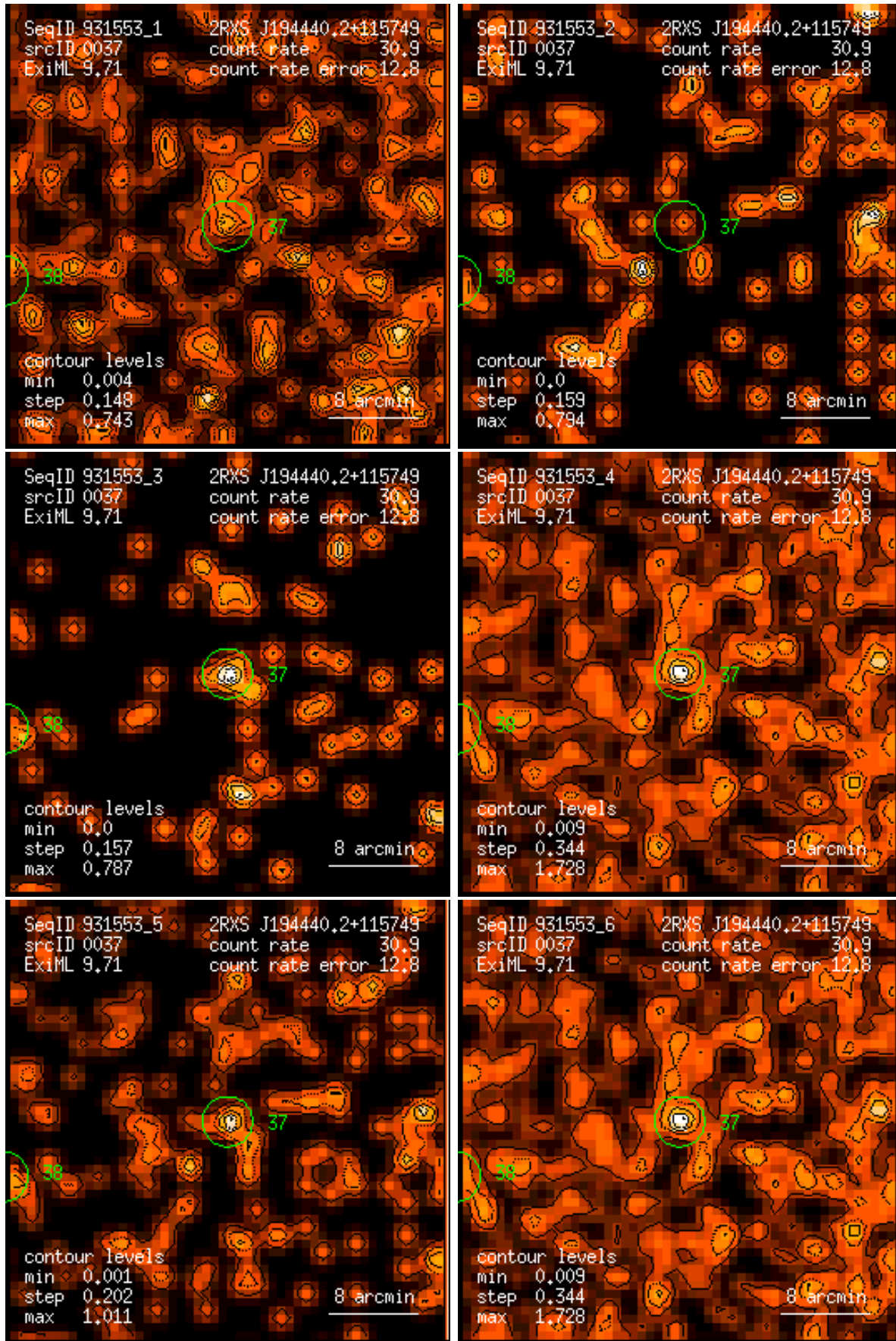
Figure 37: RASS 931553: detection 0037: band rate images, Gaussian filter: (1) PSPC channels 11 – 41, (2) 52 – 90, (3) 91 – 201, (4) 11 – 235, (5) 52 – 201, (6) 11 – 201. Broad band rates in counts/ks. Band rate contour levels in counts/ks/arcmin 2 .
