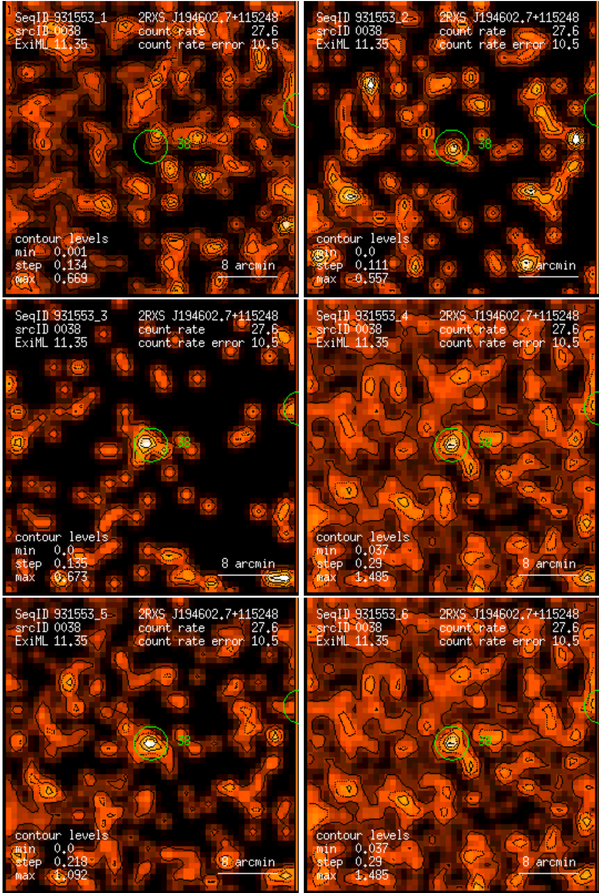
Figure 38: RASS 931553: detection 0038: band rate images, Gaussian filter: (1) PSPC channels 11 – 41, (2) 52 – 90, (3) 91 – 201, (4) 11 – 235, (5) 52 – 201, (6) 11 – 201. Broad band rates in counts/ks. Band rate contour levels in counts/ks/arcmin 2 .
