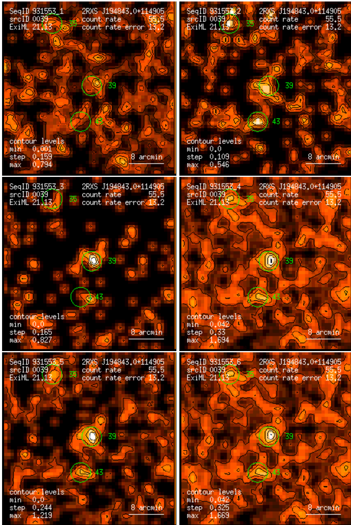
Figure 39: RASS 931553: detection 0039: band rate images, Gaussian filter: (1) PSPC channels 11 – 41, (2) 52 – 90, (3) 91 – 201, (4) 11 – 235, (5) 52 – 201, (6) 11 – 201. Broad band rates in counts/ks. Band rate contour levels in counts/ks/arcmin 2 .
