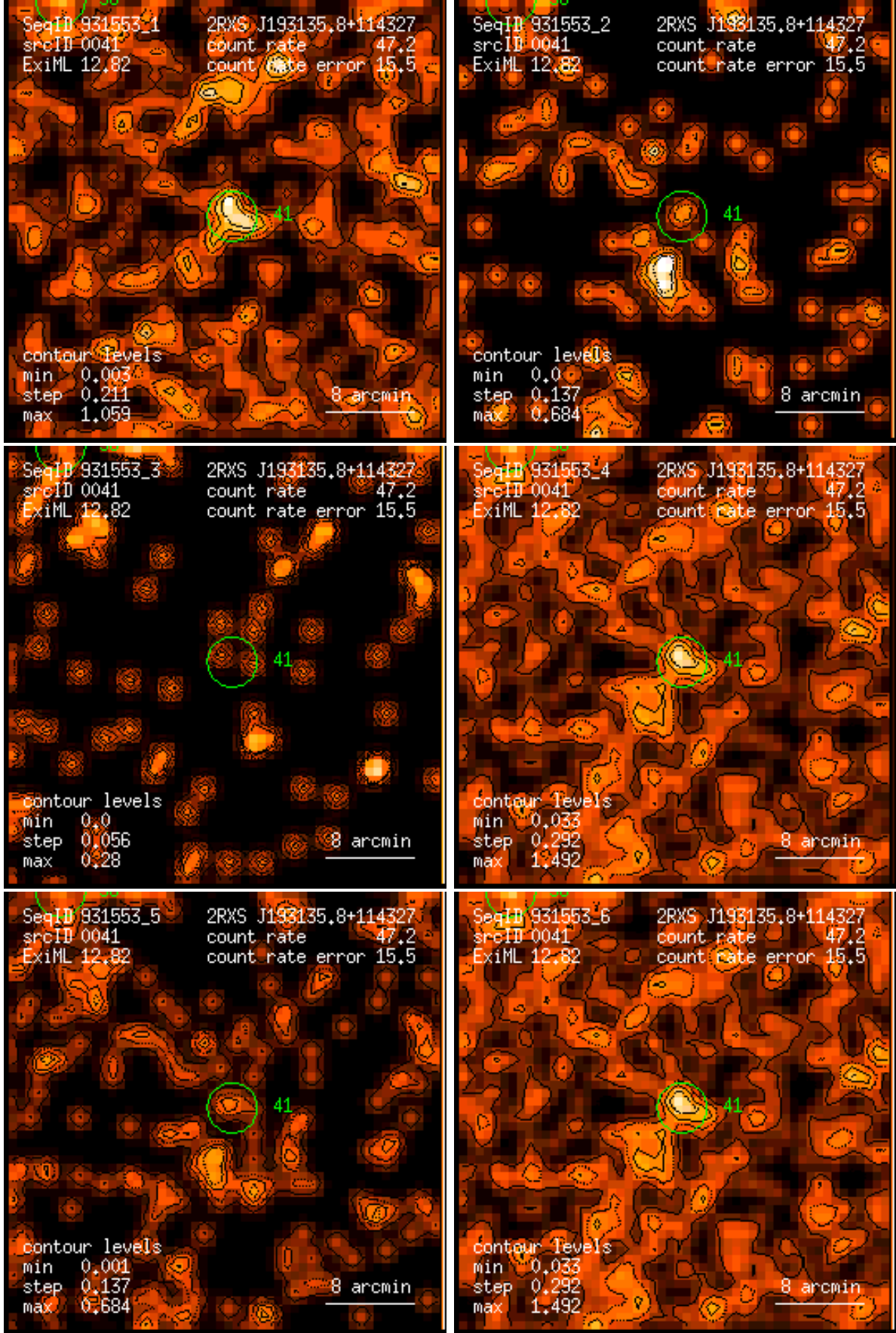
Figure 41: RASS 931553: detection 0041: band rate images, Gaussian filter: (1) PSPC channels 11 – 41, (2) 52 – 90, (3) 91 – 201, (4) 11 – 235, (5) 52 – 201, (6) 11 – 201. Broad band rates in counts/ks. Band rate contour levels in counts/ks/arcmin 2 .
