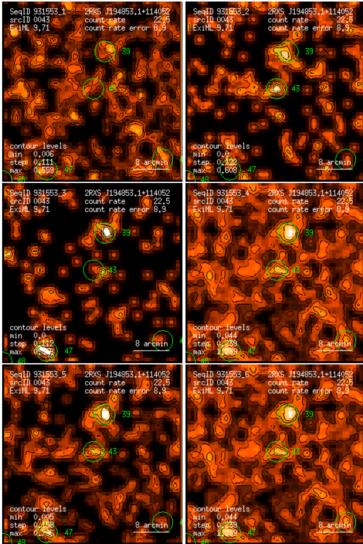
Figure 43: RASS 931553: detection 0043: band rate images, Gaussian filter: (1) PSPC channels 11 – 41, (2) 52 – 90, (3) 91 – 201, (4) 11 – 235, (5) 52 – 201, (6) 11 – 201. Broad band rates in counts/ks. Band rate contour levels in counts/ks/arcmin 2 .
