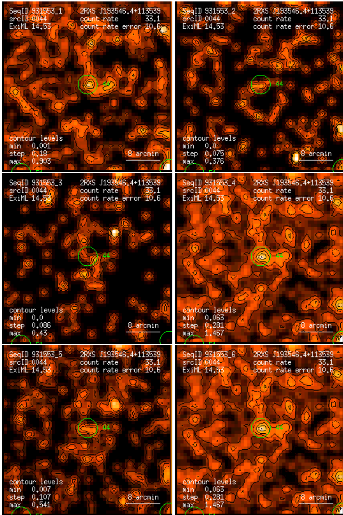
Figure 44: RASS 931553: detection 0044: band rate images, Gaussian filter: (1) PSPC channels 11 – 41, (2) 52 – 90, (3) 91 – 201, (4) 11 – 235, (5) 52 – 201, (6) 11 – 201. Broad band rates in counts/ks. Band rate contour levels in counts/ks/arcmin 2 .
