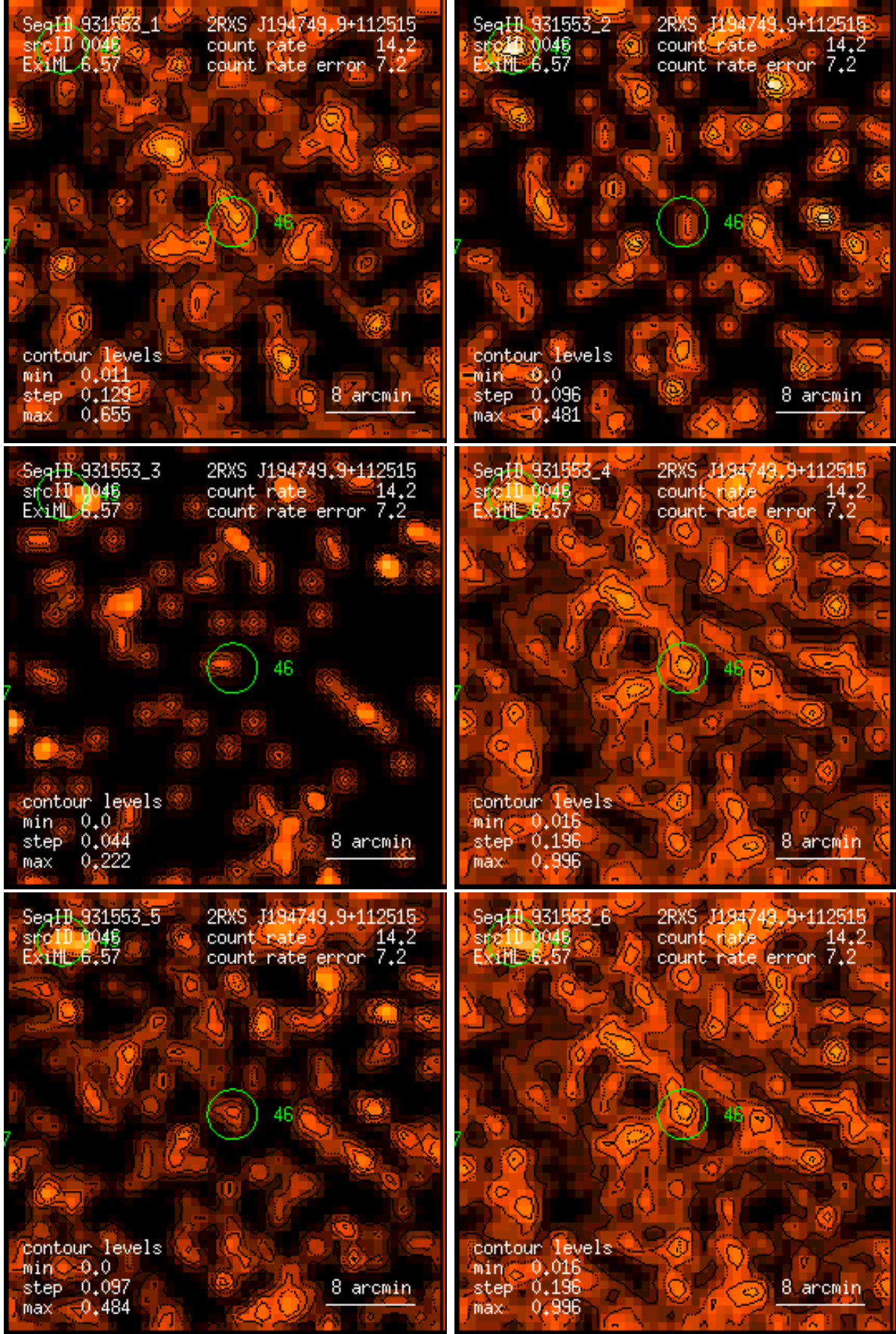
Figure 46: RASS 931553: detection 0046: band rate images, Gaussian filter: (1) PSPC channels 11 – 41, (2) 52 – 90, (3) 91 – 201, (4) 11 – 235, (5) 52 – 201, (6) 11 – 201. Broad band rates in counts/ks. Band rate contour levels in counts/ks/arcmin 2 .
