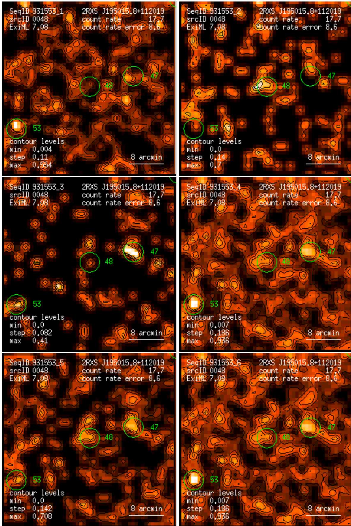
Figure 48: RASS 931553: detection 0048: band rate images, Gaussian filter: (1) PSPC channels 11 – 41, (2) 52 – 90, (3) 91 – 201, (4) 11 – 235, (5) 52 – 201, (6) 11 – 201. Broad band rates in counts/ks. Band rate contour levels in counts/ks/arcmin 2 .
