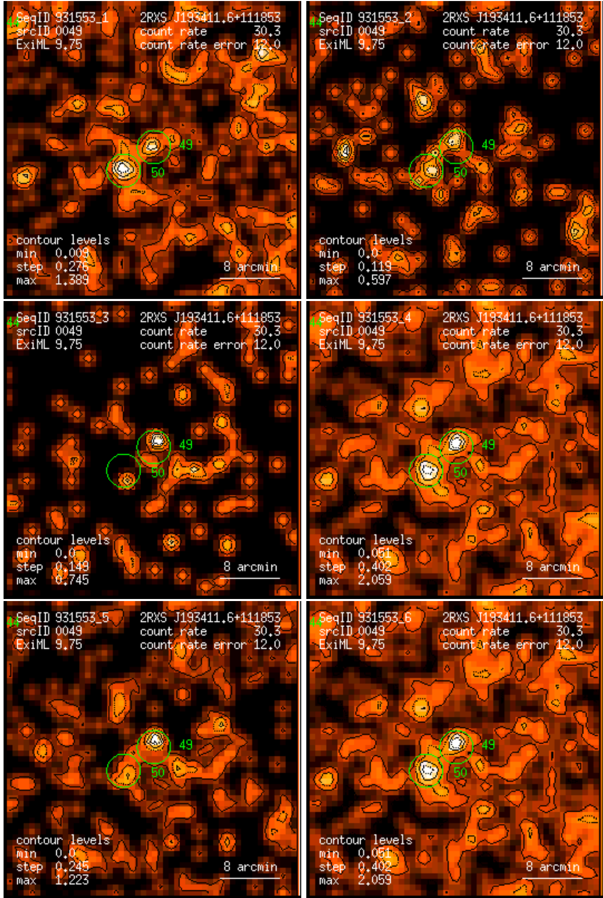
Figure 49: RASS 931553: detection 0049: band rate images, Gaussian filter: (1) PSPC channels 11 – 41, (2) 52 – 90, (3) 91 – 201, (4) 11 – 235, (5) 52 – 201, (6) 11 – 201. Broad band rates in counts/ks. Band rate contour levels in counts/ks/arcmin 2 .
