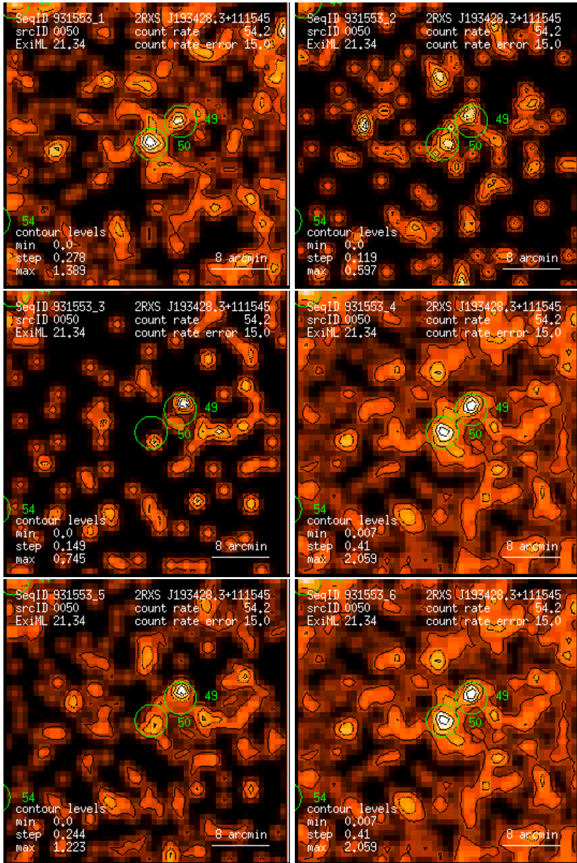
Figure 50: RASS 931553: detection 0050: band rate images, Gaussian filter: (1) PSPC channels 11 – 41, (2) 52 – 90, (3) 91 – 201, (4) 11 – 235, (5) 52 – 201, (6) 11 – 201. Broad band rates in counts/ks. Band rate contour levels in counts/ks/arcmin 2 .
