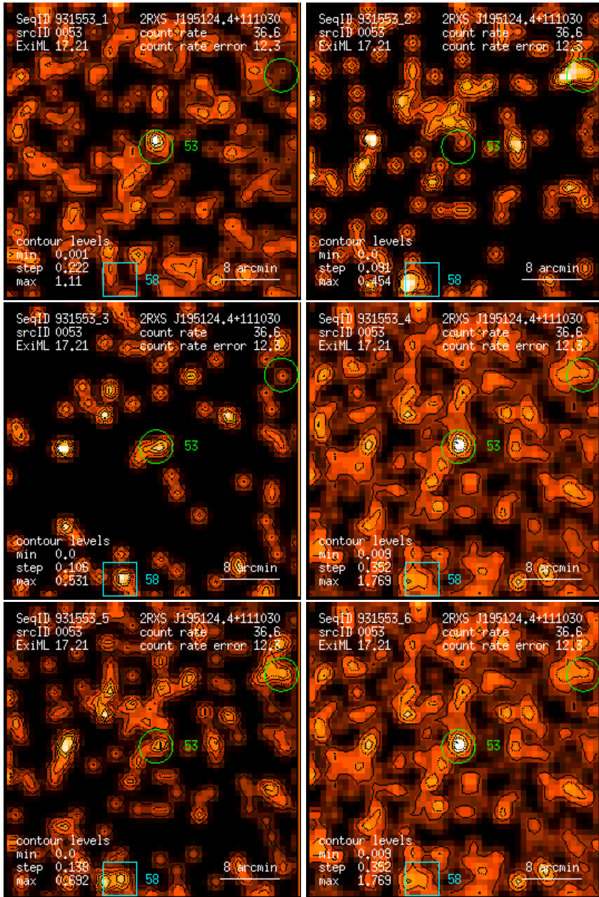
Figure 53: RASS 931553: detection 0053: band rate images, Gaussian filter: (1) PSPC channels 11 – 41, (2) 52 – 90, (3) 91 – 201, (4) 11 – 235, (5) 52 – 201, (6) 11 – 201. Broad band rates in counts/ks. Band rate contour levels in counts/ks/arcmin 2 .
