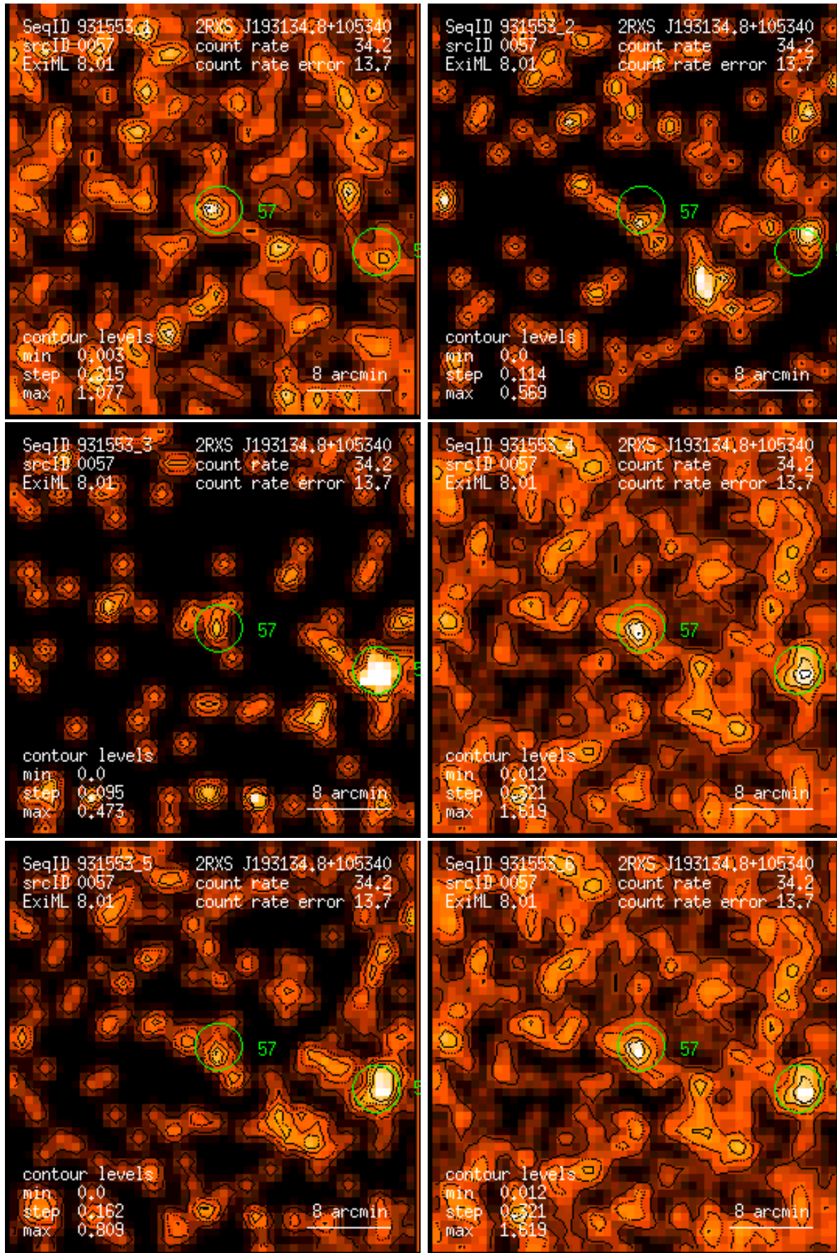
Figure 57: RASS 931553: detection 0057: band rate images, Gaussian filter: (1) PSPC channels 11 – 41, (2) 52 – 90, (3) 91 – 201, (4) 11 – 235, (5) 52 – 201, (6) 11 – 201. Broad band rates in counts/ks. Band rate contour levels in counts/ks/arcmin 2 .
