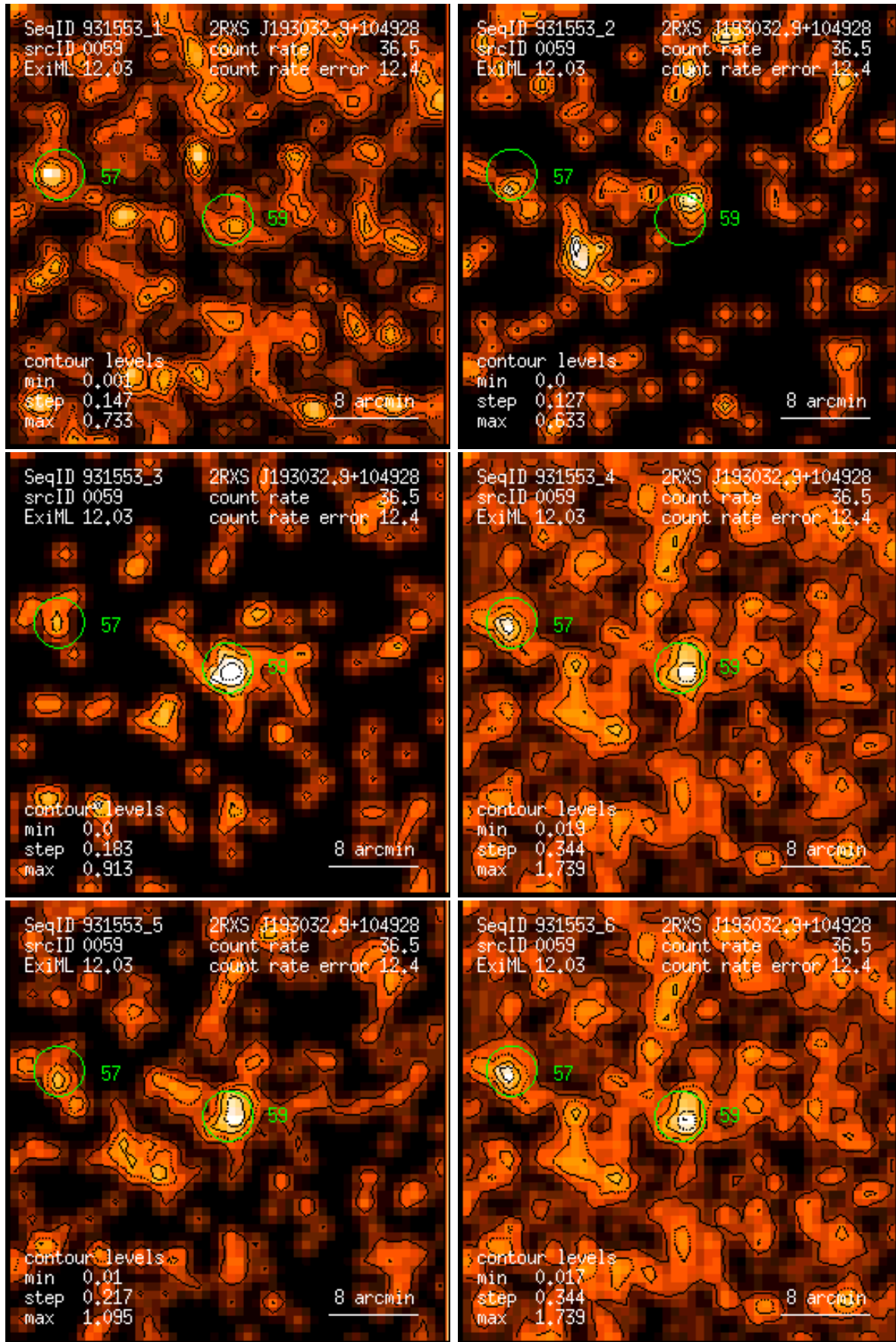
Figure 59: RASS 931553: detection 0059: band rate images, Gaussian filter: (1) PSPC channels 11 – 41, (2) 52 – 90, (3) 91 – 201, (4) 11 – 235, (5) 52 – 201, (6) 11 – 201. Broad band rates in counts/ks. Band rate contour levels in counts/ks/arcmin 2 .
