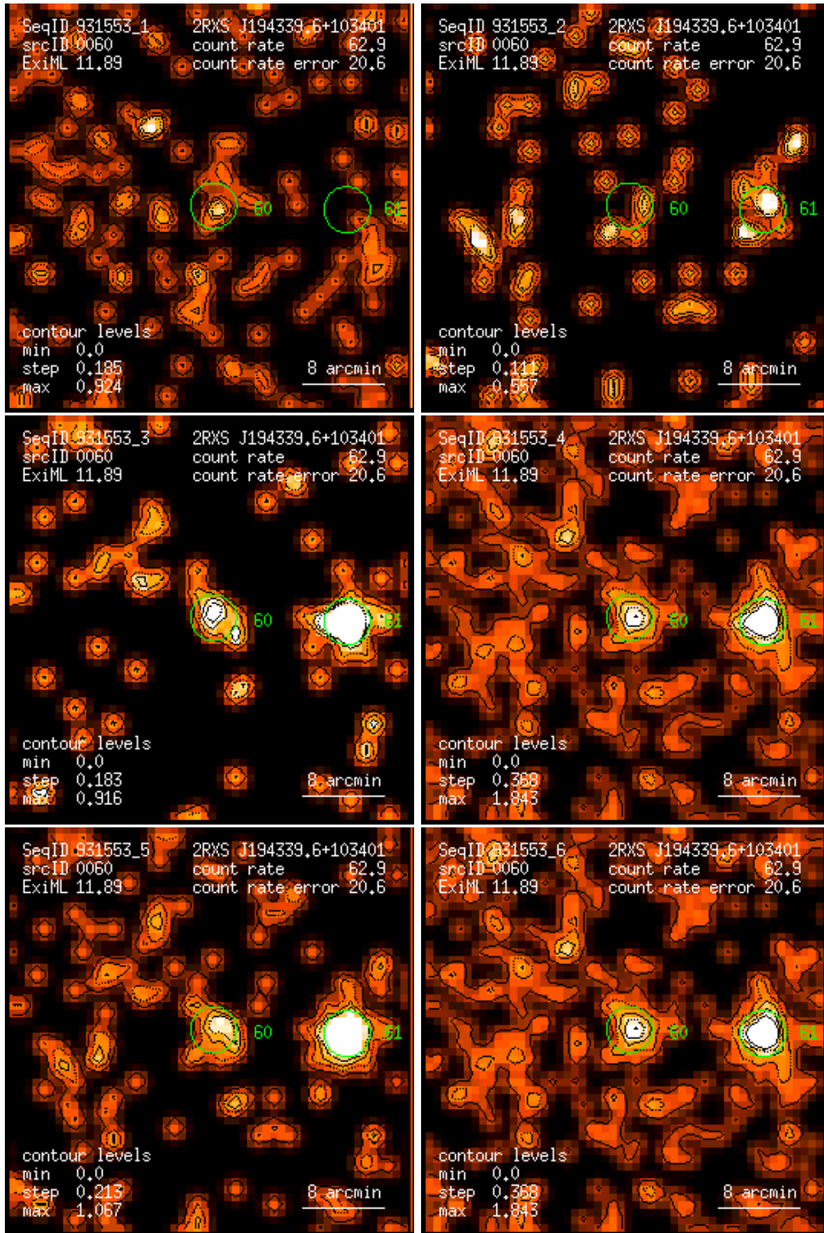
Figure 60: RASS 931553: detection 0060: band rate images, Gaussian filter: (1) PSPC channels 11 – 41, (2) 52 – 90, (3) 91 – 201, (4) 11 – 235, (5) 52 – 201, (6) 11 – 201. Broad band rates in counts/ks. Band rate contour levels in counts/ks/arcmin 2 .
