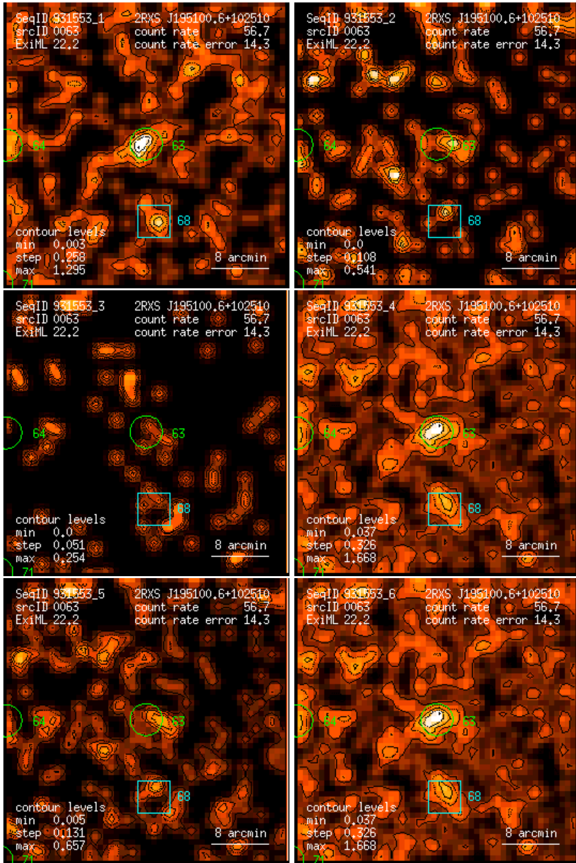
Figure 63: RASS 931553: detection 0063: band rate images, Gaussian filter: (1) PSPC channels 11 – 41, (2) 52 – 90, (3) 91 – 201, (4) 11 – 235, (5) 52 – 201, (6) 11 – 201. Broad band rates in counts/ks. Band rate contour levels in counts/ks/arcmin 2 .
