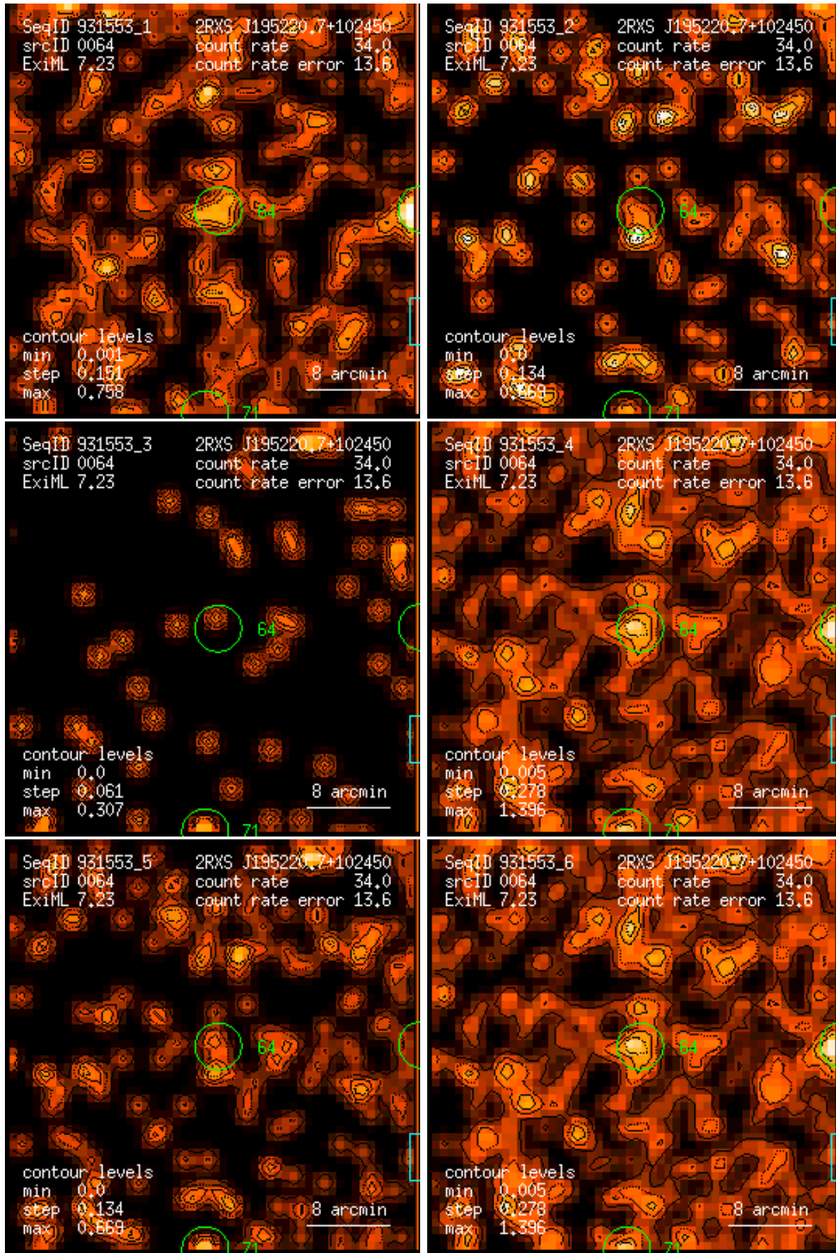
Figure 64: RASS 931553: detection 0064: band rate images, Gaussian filter: (1) PSPC channels 11 – 41, (2) 52 – 90, (3) 91 – 201, (4) 11 – 235, (5) 52 – 201, (6) 11 – 201. Broad band rates in counts/ks. Band rate contour levels in counts/ks/arcmin 2 .
