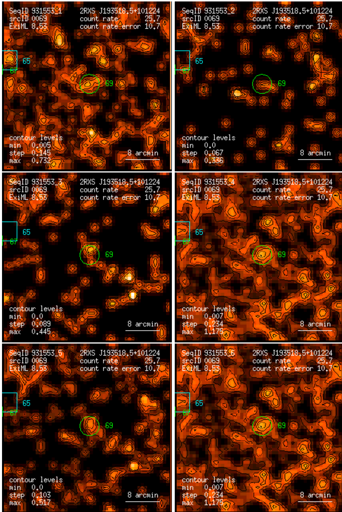
Figure 69: RASS 931553: detection 0069: band rate images, Gaussian filter: (1) PSPC channels 11 – 41, (2) 52 – 90, (3) 91 – 201, (4) 11 – 235, (5) 52 – 201, (6) 11 – 201. Broad band rates in counts/ks. Band rate contour levels in counts/ks/arcmin 2 .
