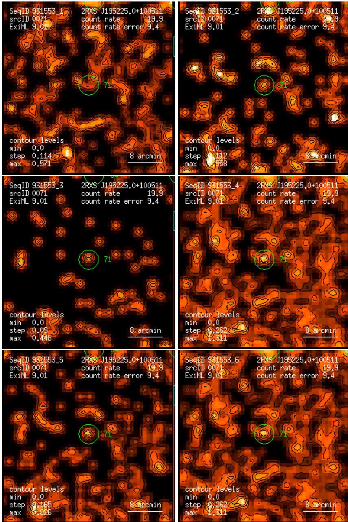
Figure 71: RASS 931553: detection 0071: band rate images, Gaussian filter: (1) PSPC channels 11 – 41, (2) 52 – 90, (3) 91 – 201, (4) 11 – 235, (5) 52 – 201, (6) 11 – 201. Broad band rates in counts/ks. Band rate contour levels in counts/ks/arcmin 2 .
