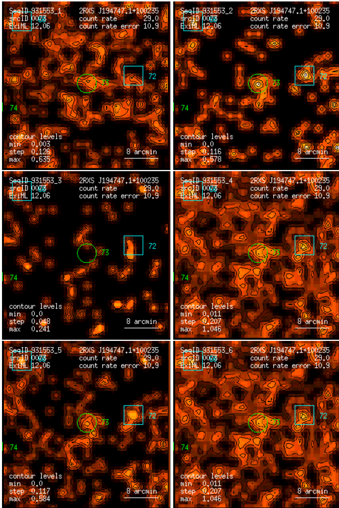
Figure 73: RASS 931553: detection 0073: band rate images, Gaussian filter: (1) PSPC channels 11 – 41, (2) 52 – 90, (3) 91 – 201, (4) 11 – 235, (5) 52 – 201, (6) 11 – 201. Broad band rates in counts/ks. Band rate contour levels in counts/ks/arcmin 2 .
