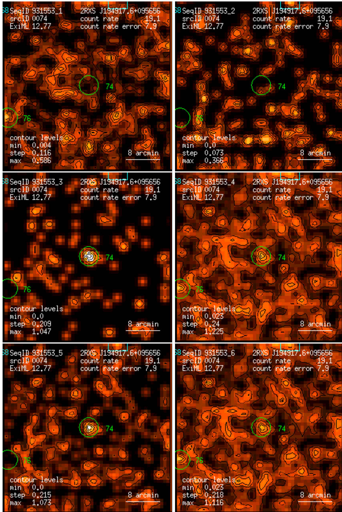
Figure 74: RASS 931553: detection 0074: band rate images, Gaussian filter: (1) PSPC channels 11 – 41, (2) 52 – 90, (3) 91 – 201, (4) 11 – 235, (5) 52 – 201, (6) 11 – 201. Broad band rates in counts/ks. Band rate contour levels in counts/ks/arcmin 2 .
