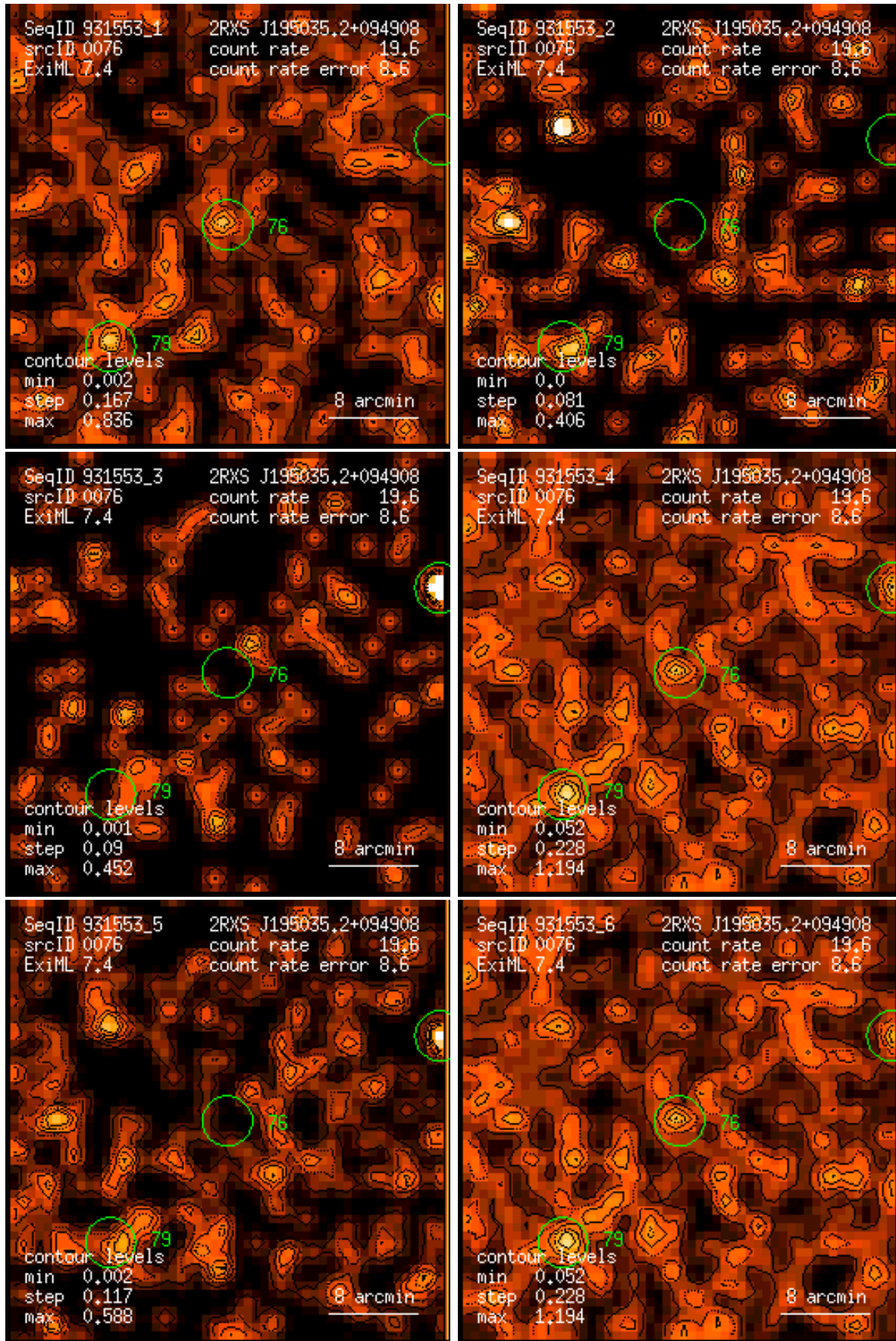
Figure 76: RASS 931553: detection 0076: band rate images, Gaussian filter: (1) PSPC channels 11 – 41, (2) 52 – 90, (3) 91 – 201, (4) 11 – 235, (5) 52 – 201, (6) 11 – 201. Broad band rates in counts/ks. Band rate contour levels in counts/ks/arcmin 2 .
