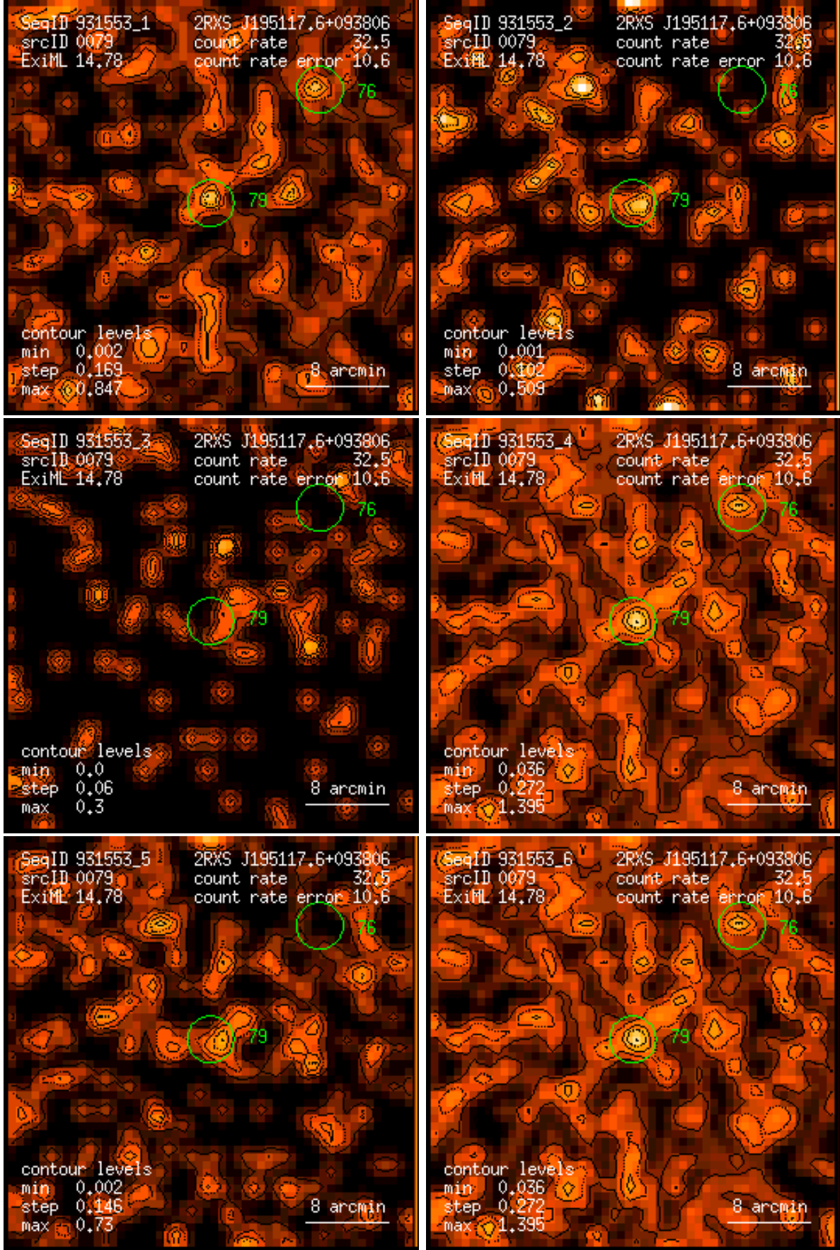
Figure 79: RASS 931553: detection 0079: band rate images, Gaussian filter: (1) PSPC channels 11 – 41, (2) 52 – 90, (3) 91 – 201, (4) 11 – 235, (5) 52 – 201, (6) 11 – 201. Broad band rates in counts/ks. Band rate contour levels in counts/ks/arcmin 2 .
