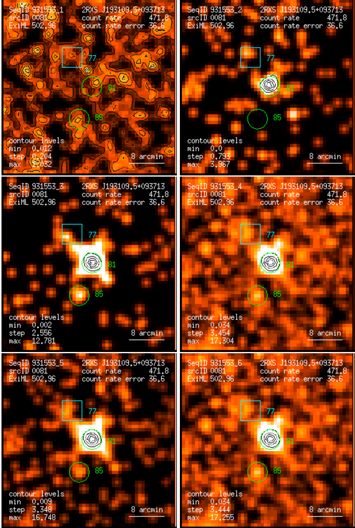
Figure 81: RASS 931553: detection 0081: band rate images, Gaussian filter: (1) PSPC channels 11 – 41, (2) 52 – 90, (3) 91 – 201, (4) 11 – 235, (5) 52 – 201, (6) 11 – 201. Broad band rates in counts/ks. Band rate contour levels in counts/ks/arcmin 2 .
