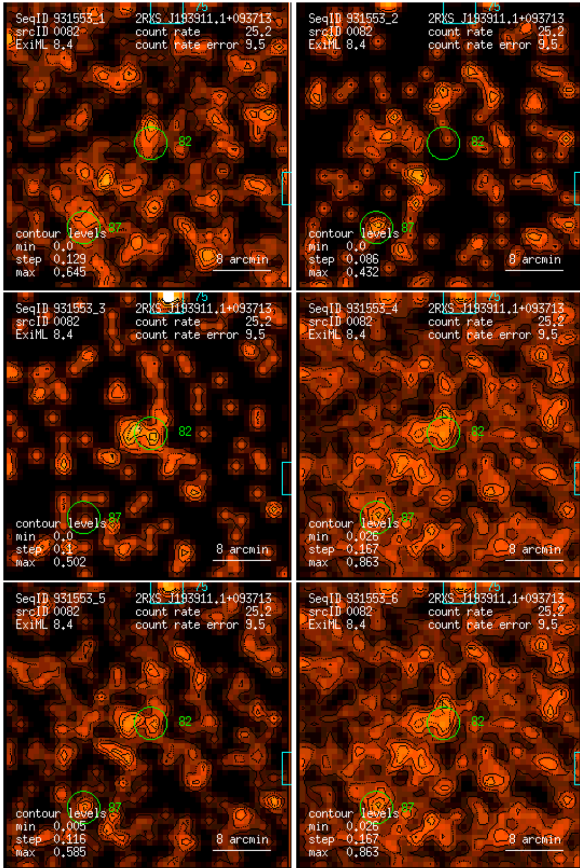
Figure 82: RASS 931553: detection 0082: band rate images, Gaussian filter: (1) PSPC channels 11 – 41, (2) 52 – 90, (3) 91 – 201, (4) 11 – 235, (5) 52 – 201, (6) 11 – 201. Broad band rates in counts/ks. Band rate contour levels in counts/ks/arcmin 2 .
