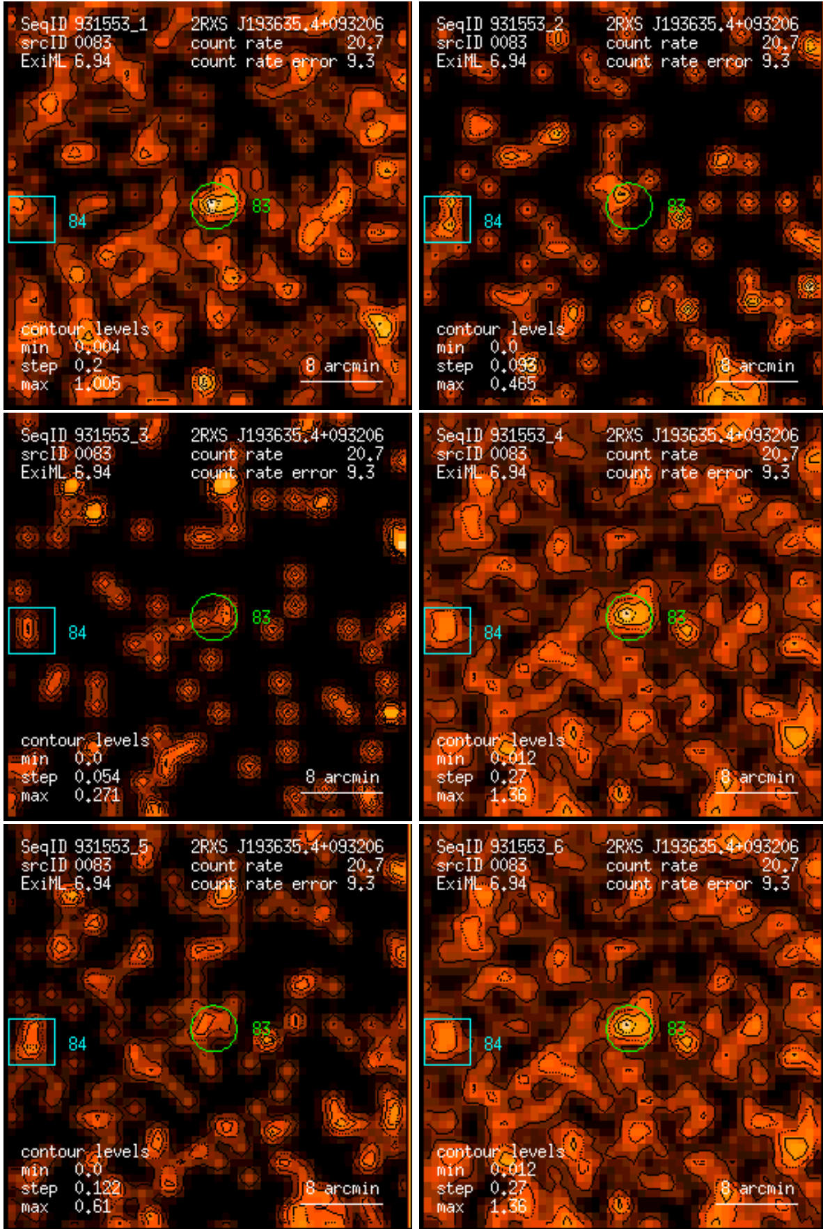
Figure 83: RASS 931553: detection 0083: band rate images, Gaussian filter: (1) PSPC channels 11 – 41, (2) 52 – 90, (3) 91 – 201, (4) 11 – 235, (5) 52 – 201, (6) 11 – 201. Broad band rates in counts/ks. Band rate contour levels in counts/ks/arcmin 2 .
