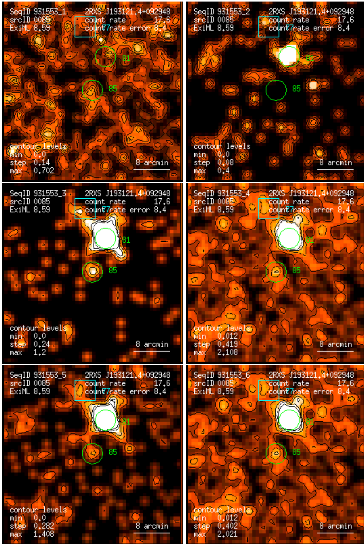
Figure 85: RASS 931553: detection 0085: band rate images, Gaussian filter: (1) PSPC channels 11 – 41, (2) 52 – 90, (3) 91 – 201, (4) 11 – 235, (5) 52 – 201, (6) 11 – 201. Broad band rates in counts/ks. Band rate contour levels in counts/ks/arcmin 2 .
