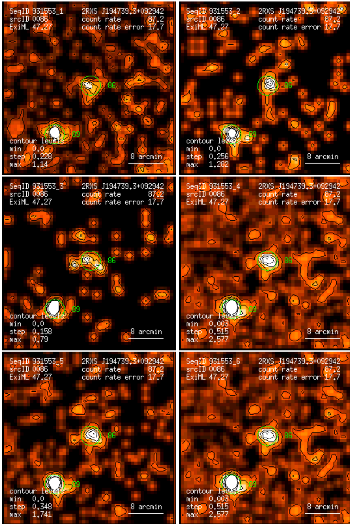
Figure 86: RASS 931553: detection 0086: band rate images, Gaussian filter: (1) PSPC channels 11 – 41, (2) 52 – 90, (3) 91 – 201, (4) 11 – 235, (5) 52 – 201, (6) 11 – 201. Broad band rates in counts/ks. Band rate contour levels in counts/ks/arcmin 2 .
