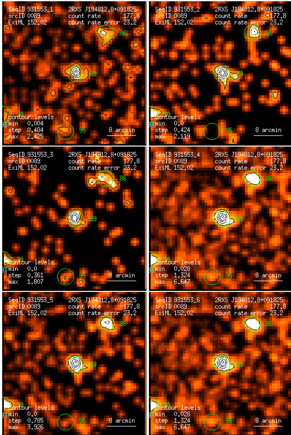
Figure 89: RASS 931553: detection 0089: band rate images, Gaussian filter: (1) PSPC channels 11 – 41, (2) 52 – 90, (3) 91 – 201, (4) 11 – 235, (5) 52 – 201, (6) 11 – 201. Broad band rates in counts/ks. Band rate contour levels in counts/ks/arcmin 2 .
