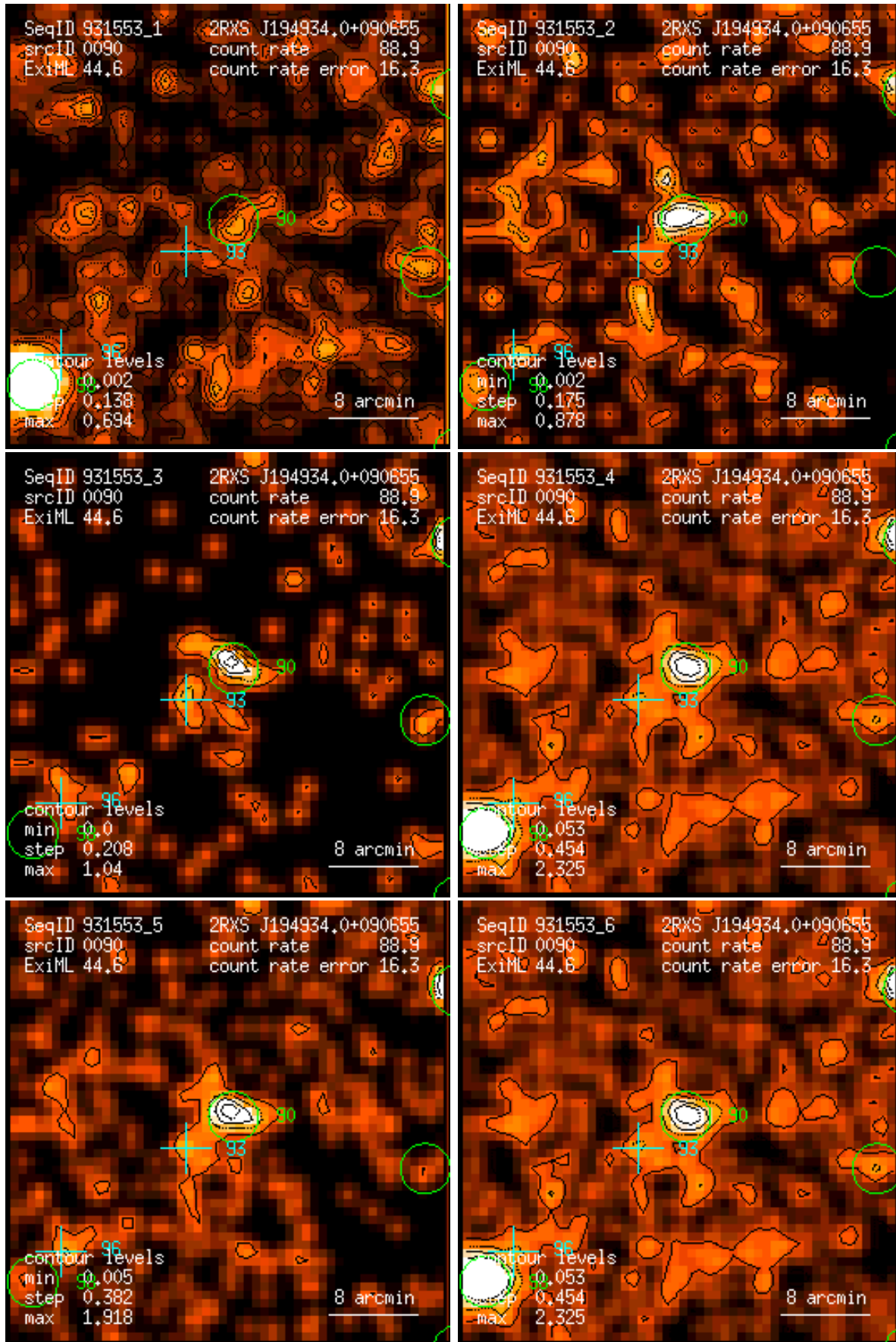
Figure 90: RASS 931553: detection 0090: band rate images, Gaussian filter: (1) PSPC channels 11 – 41, (2) 52 – 90, (3) 91 – 201, (4) 11 – 235, (5) 52 – 201, (6) 11 – 201. Broad band rates in counts/ks. Band rate contour levels in counts/ks/arcmin 2 .
