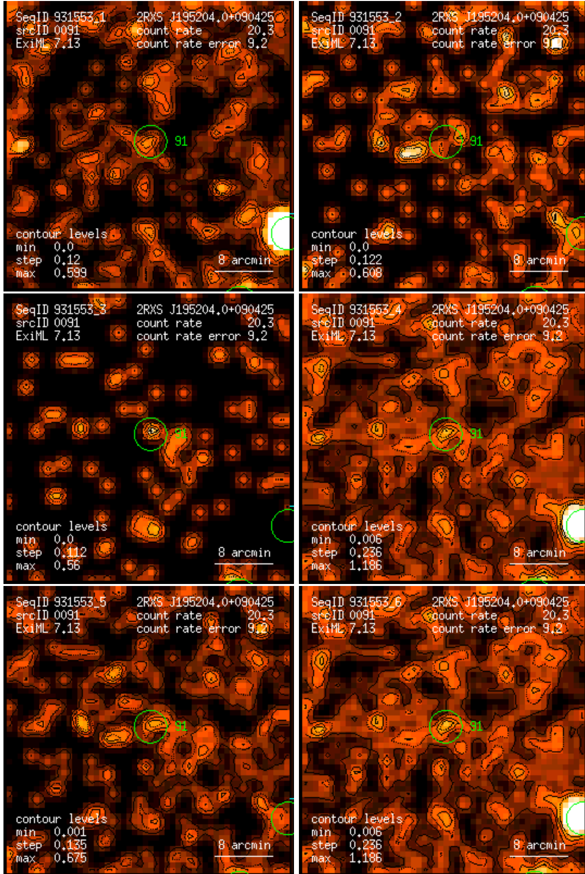
Figure 91: RASS 931553: detection 0091: band rate images, Gaussian filter: (1) PSPC channels 11 – 41, (2) 52 – 90, (3) 91 – 201, (4) 11 – 235, (5) 52 – 201, (6) 11 – 201. Broad band rates in counts/ks. Band rate contour levels in counts/ks/arcmin 2 .
